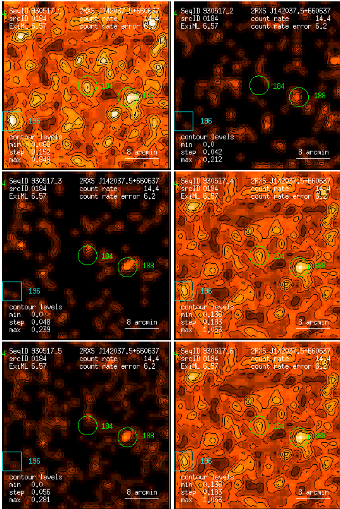
Figure 184: RASS 930517: detection 0184: band rate images, Gaussian filter: (1) PSPC channels 11 – 41, (2) 52 – 90, (3) 91 – 201, (4) 11 – 235, (5) 52 – 201, (6) 11 – 201. Broad band rates in counts/ks. Band rate contour levels in counts/ks/arcmin 2 .
