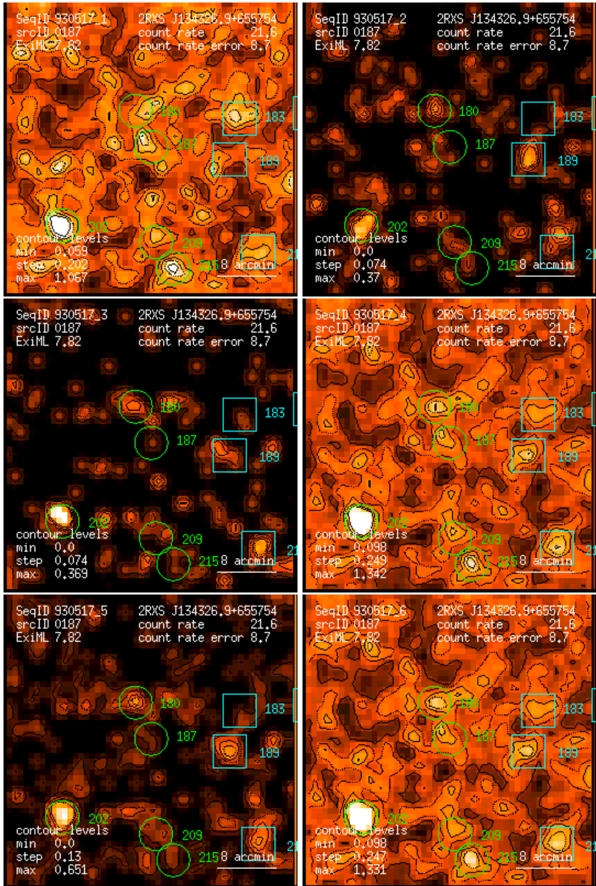
Figure 187: RASS 930517: detection 0187: band rate images, Gaussian filter: (1) PSPC channels 11 – 41, (2) 52 – 90, (3) 91 – 201, (4) 11 – 235, (5) 52 – 201, (6) 11 – 201. Broad band rates in counts/ks. Band rate contour levels in counts/ks/arcmin 2 .
