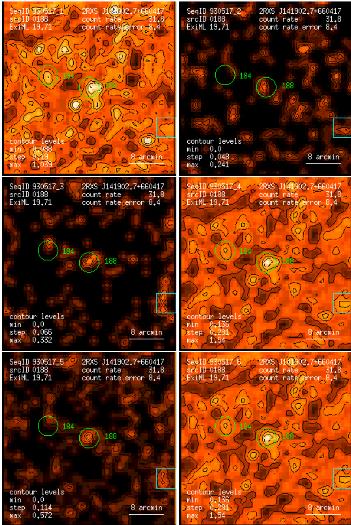
Figure 188: RASS 930517: detection 0188: band rate images, Gaussian filter: (1) PSPC channels 11 – 41, (2) 52 – 90, (3) 91 – 201, (4) 11 – 235, (5) 52 – 201, (6) 11 – 201. Broad band rates in counts/ks. Band rate contour levels in counts/ks/arcmin 2 .
