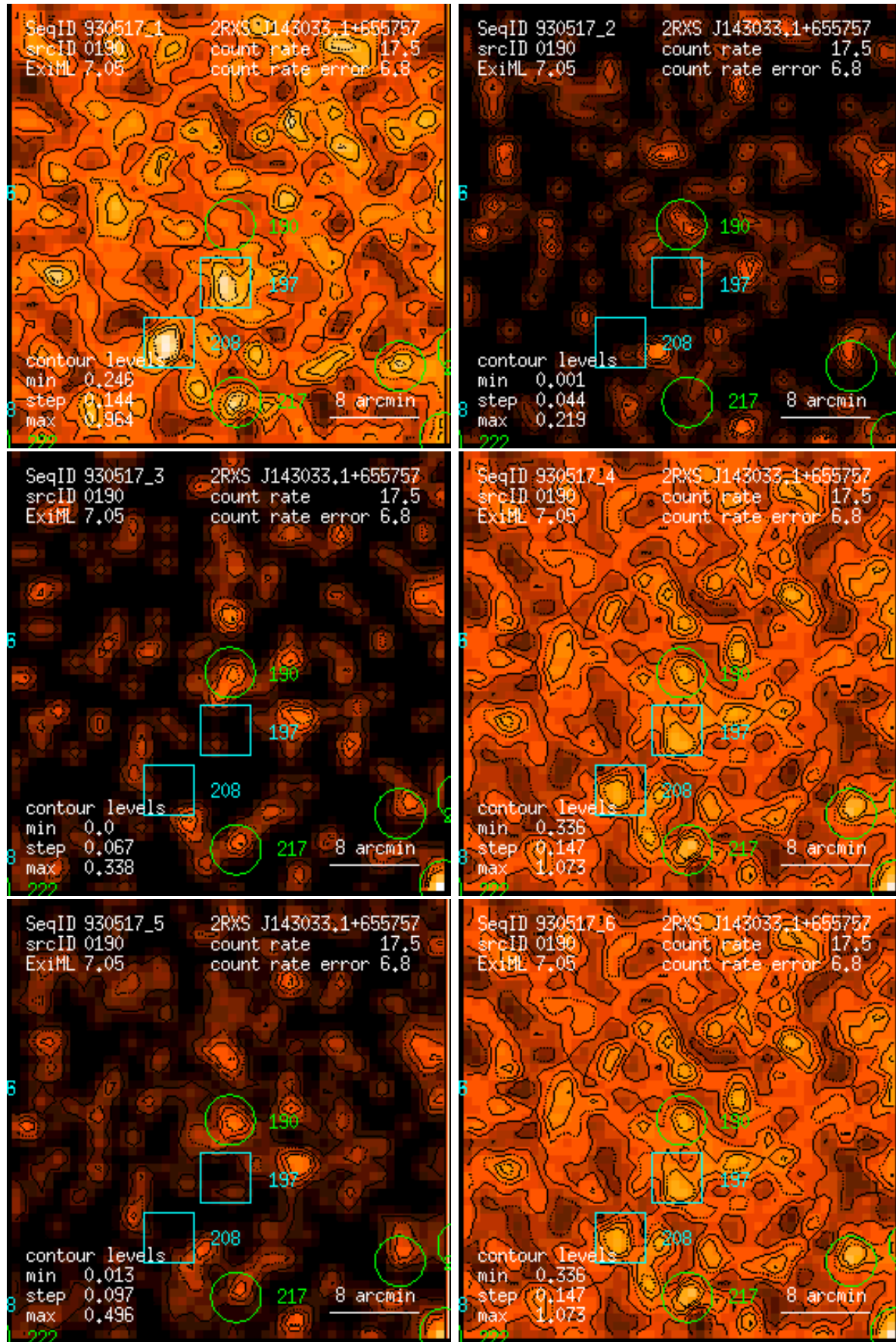
Figure 190: RASS 930517: detection 0190: band rate images, Gaussian filter: (1) PSPC channels 11 – 41, (2) 52 – 90, (3) 91 – 201, (4) 11 – 235, (5) 52 – 201, (6) 11 – 201. Broad band rates in counts/ks. Band rate contour levels in counts/ks/arcmin 2 .
