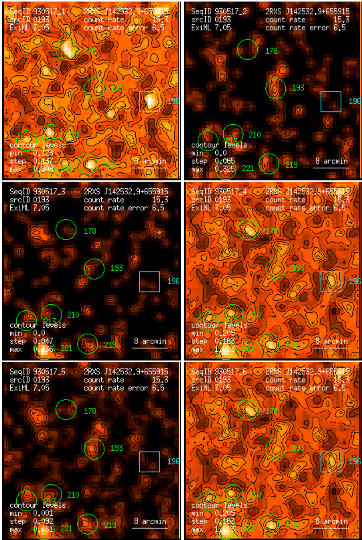
Figure 193: RASS 930517: detection 0193: band rate images, Gaussian filter: (1) PSPC channels 11 – 41, (2) 52 – 90, (3) 91 – 201, (4) 11 – 235, (5) 52 – 201, (6) 11 – 201. Broad band rates in counts/ks. Band rate contour levels in counts/ks/arcmin 2 .
