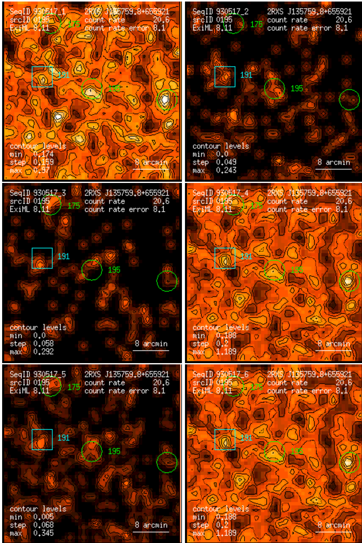
Figure 195: RASS 930517: detection 0195: band rate images, Gaussian filter: (1) PSPC channels 11 – 41, (2) 52 – 90, (3) 91 – 201, (4) 11 – 235, (5) 52 – 201, (6) 11 – 201. Broad band rates in counts/ks. Band rate contour levels in counts/ks/arcmin 2 .
