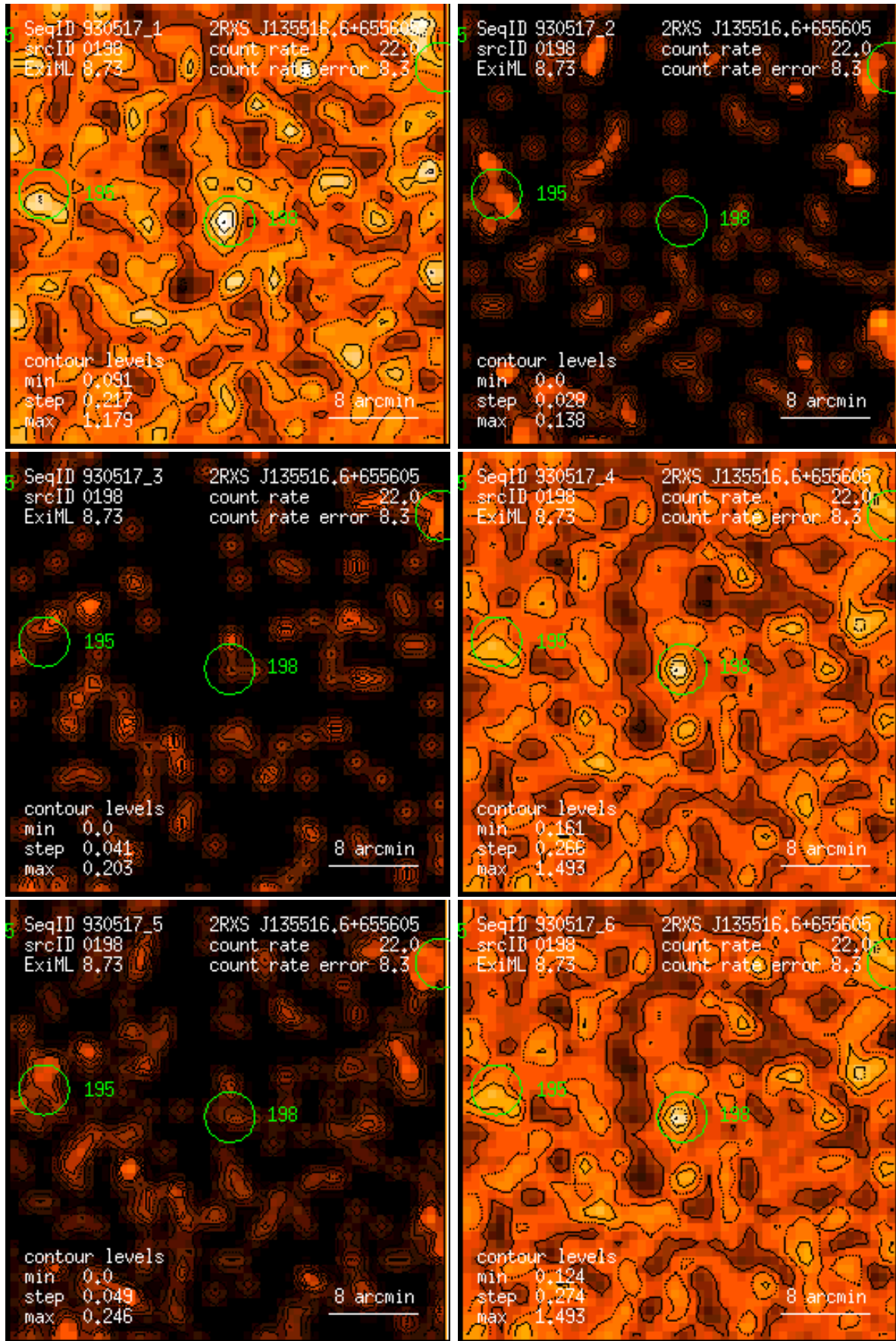
Figure 198: RASS 930517: detection 0198: band rate images, Gaussian filter: (1) PSPC channels 11 – 41, (2) 52 – 90, (3) 91 – 201, (4) 11 – 235, (5) 52 – 201, (6) 11 – 201. Broad band rates in counts/ks. Band rate contour levels in counts/ks/arcmin 2 .
