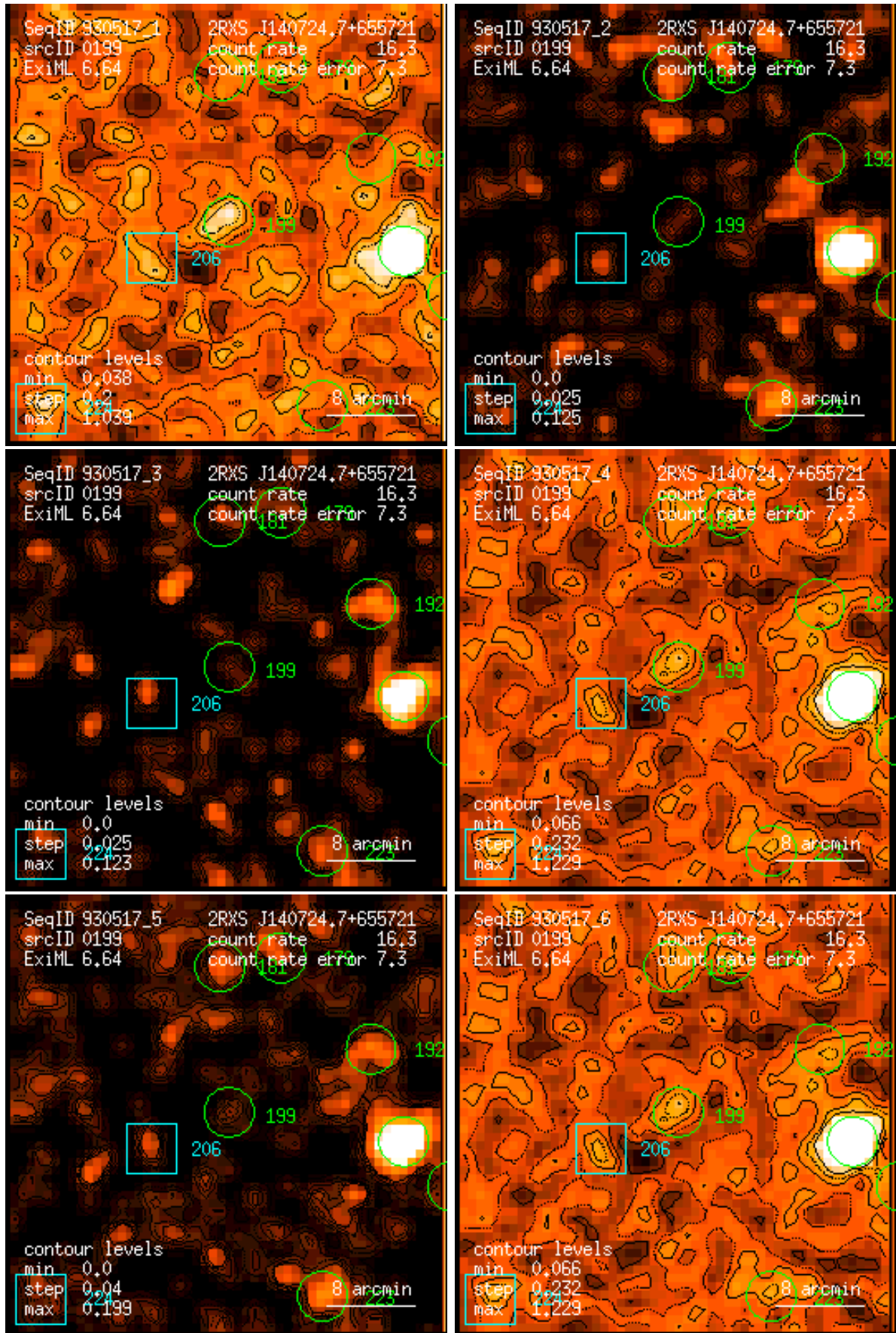
Figure 199: RASS 930517: detection 0199: band rate images, Gaussian filter: (1) PSPC channels 11 – 41, (2) 52 – 90, (3) 91 – 201, (4) 11 – 235, (5) 52 – 201, (6) 11 – 201. Broad band rates in counts/ks. Band rate contour levels in counts/ks/arcmin 2 .
