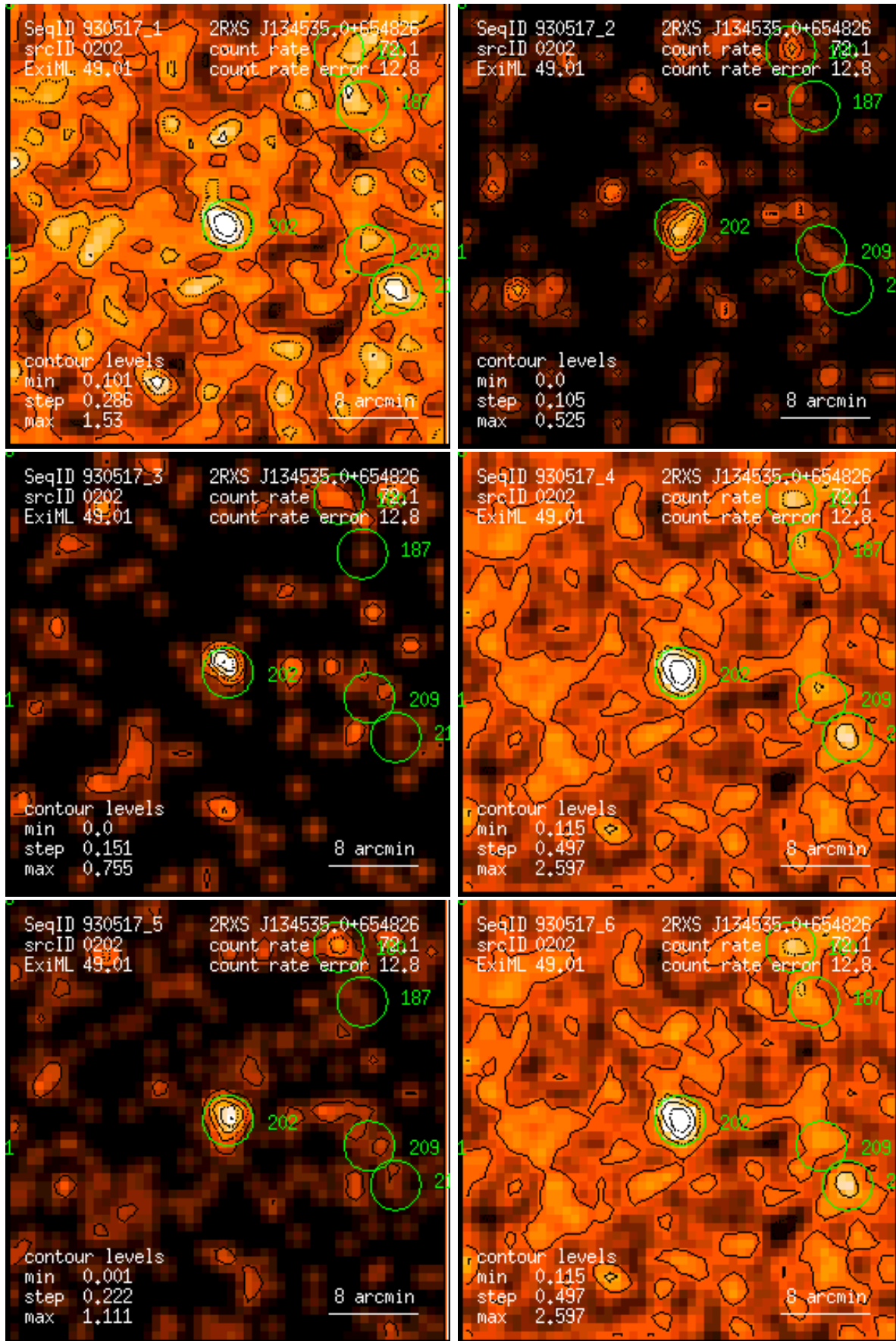
Figure 202: RASS 930517: detection 0202: band rate images, Gaussian filter: (1) PSPC channels 11 – 41, (2) 52 – 90, (3) 91 – 201, (4) 11 – 235, (5) 52 – 201, (6) 11 – 201. Broad band rates in counts/ks. Band rate contour levels in counts/ks/arcmin 2 .
