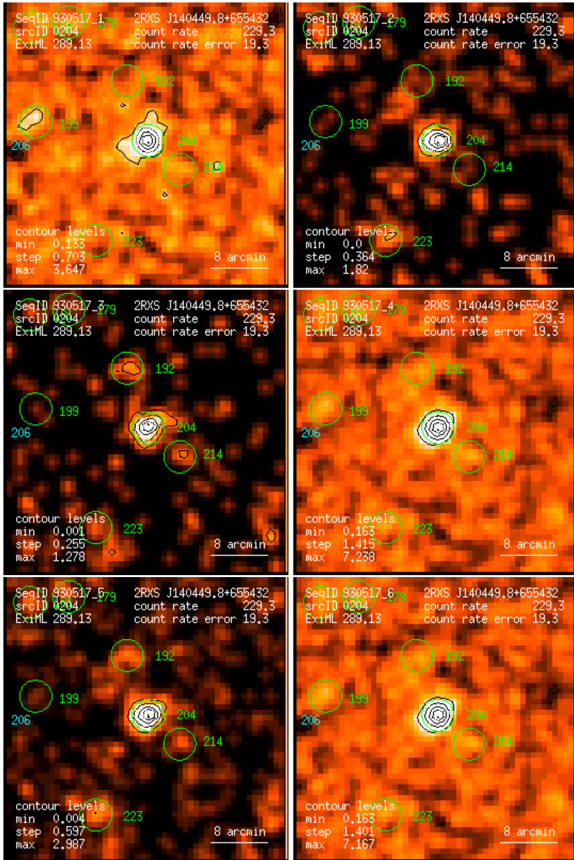
Figure 204: RASS 930517: detection 0204: band rate images, Gaussian filter: (1) PSPC channels 11 – 41, (2) 52 – 90, (3) 91 – 201, (4) 11 – 235, (5) 52 – 201, (6) 11 – 201. Broad band rates in counts/ks. Band rate contour levels in counts/ks/arcmin 2 .
