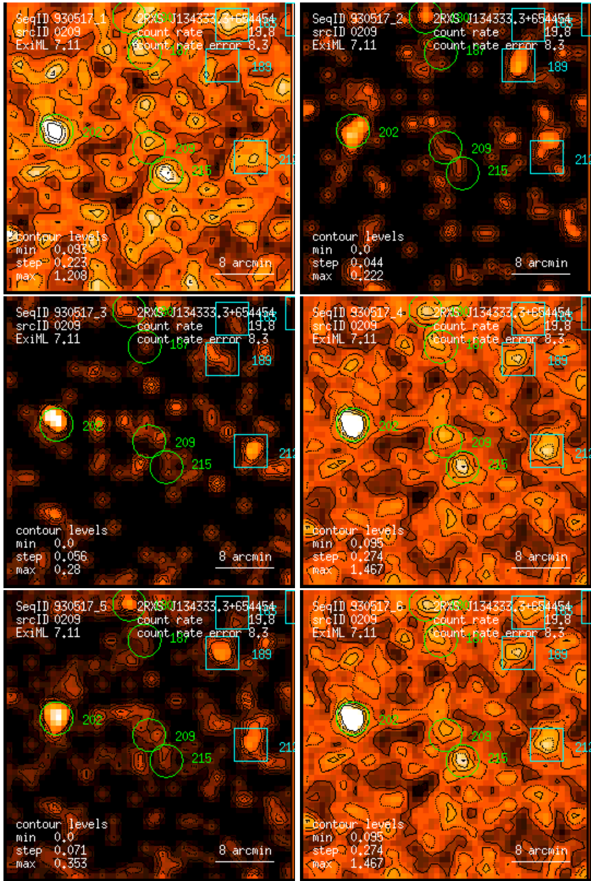
Figure 209: RASS 930517: detection 0209: band rate images, Gaussian filter: (1) PSPC channels 11 – 41, (2) 52 – 90, (3) 91 – 201, (4) 11 – 235, (5) 52 – 201, (6) 11 – 201. Broad band rates in counts/ks. Band rate contour levels in counts/ks/arcmin 2 .
