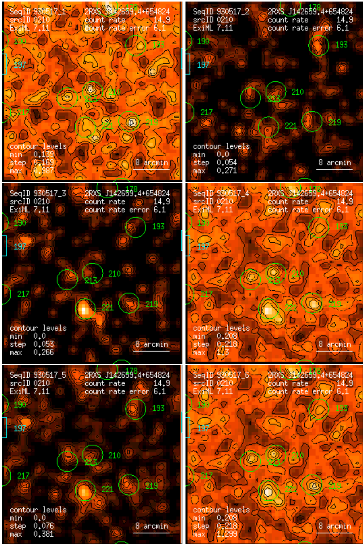
Figure 210: RASS 930517: detection 0210: band rate images, Gaussian filter: (1) PSPC channels 11 – 41, (2) 52 – 90, (3) 91 – 201, (4) 11 – 235, (5) 52 – 201, (6) 11 – 201. Broad band rates in counts/ks. Band rate contour levels in counts/ks/arcmin 2 .
