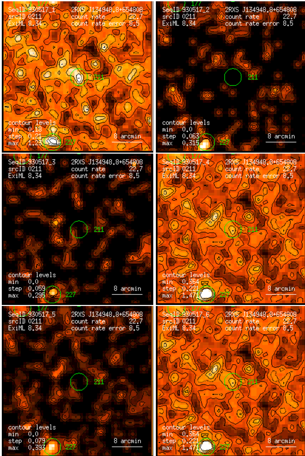
Figure 211: RASS 930517: detection 0211: band rate images, Gaussian filter: (1) PSPC channels 11 – 41, (2) 52 – 90, (3) 91 – 201, (4) 11 – 235, (5) 52 – 201, (6) 11 – 201. Broad band rates in counts/ks. Band rate contour levels in counts/ks/arcmin 2 .
