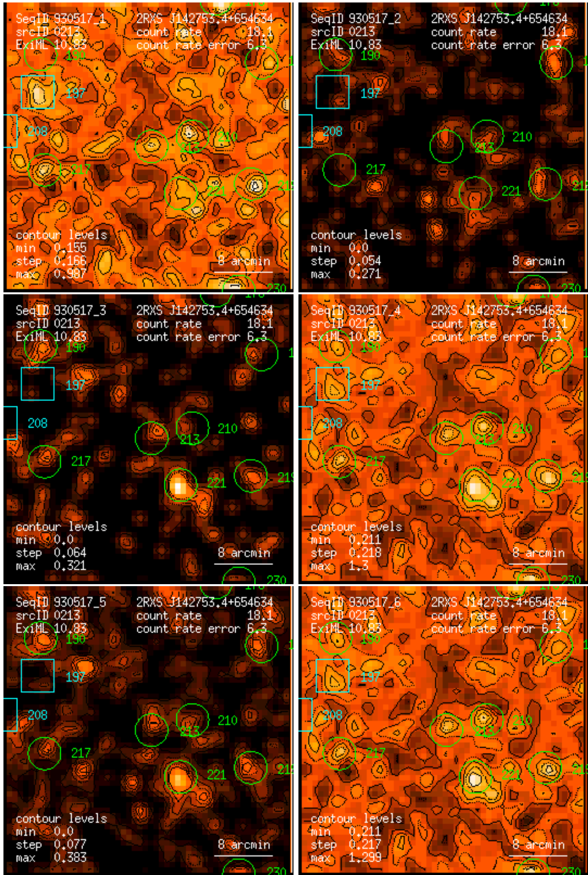
Figure 213: RASS 930517: detection 0213: band rate images, Gaussian filter: (1) PSPC channels 11 – 41, (2) 52 – 90, (3) 91 – 201, (4) 11 – 235, (5) 52 – 201, (6) 11 – 201. Broad band rates in counts/ks. Band rate contour levels in counts/ks/arcmin 2 .
