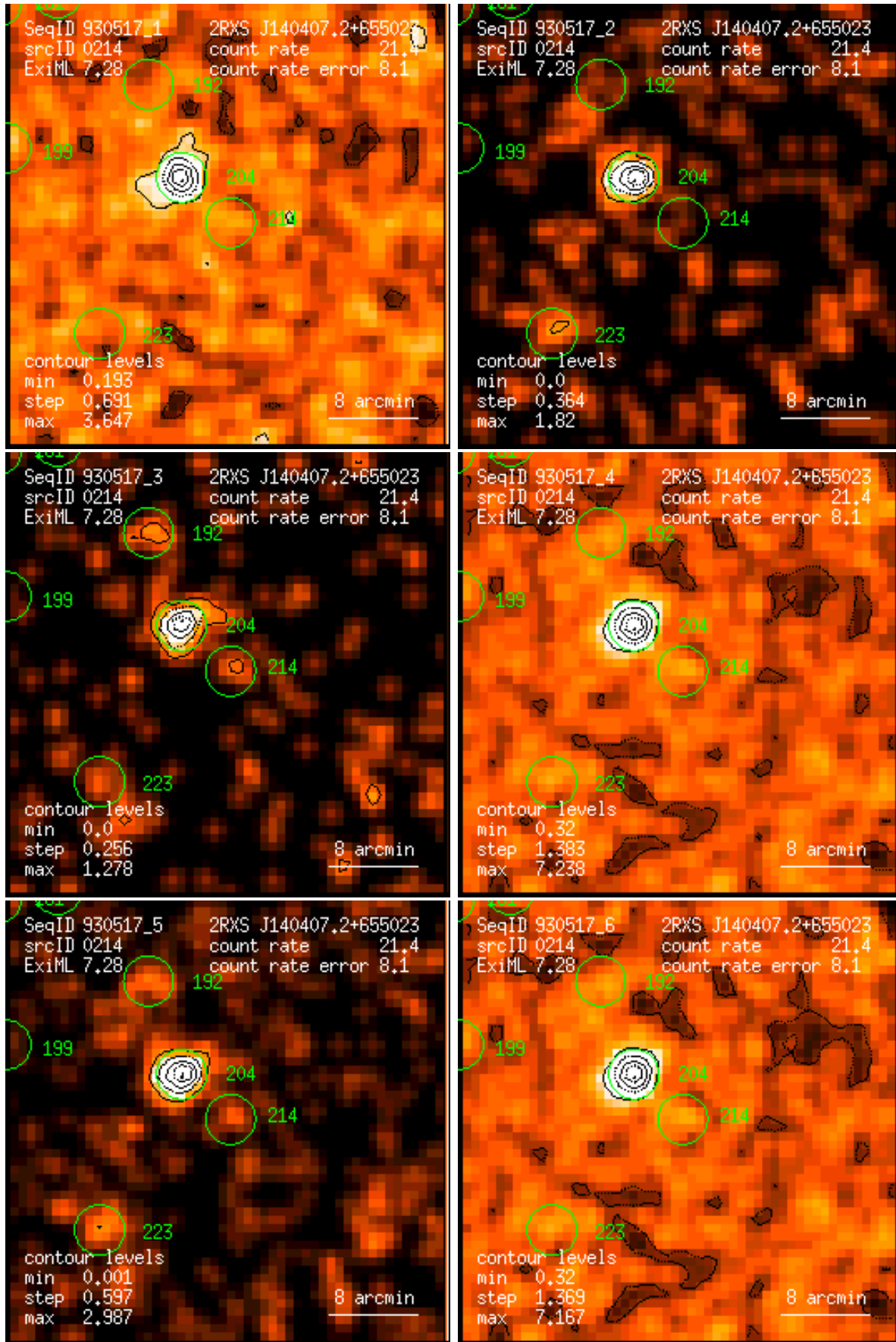
Figure 214: RASS 930517: detection 0214: band rate images, Gaussian filter: (1) PSPC channels 11 – 41, (2) 52 – 90, (3) 91 – 201, (4) 11 – 235, (5) 52 – 201, (6) 11 – 201. Broad band rates in counts/ks. Band rate contour levels in counts/ks/arcmin 2 .
