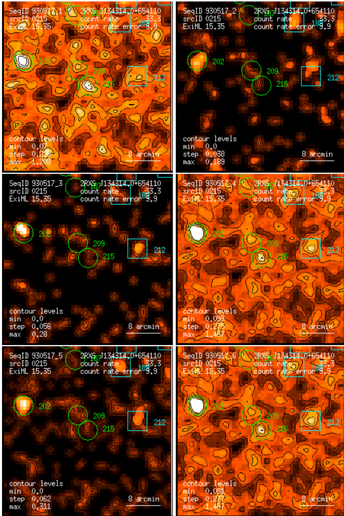
Figure 215: RASS 930517: detection 0215: band rate images, Gaussian filter: (1) PSPC channels 11 – 41, (2) 52 – 90, (3) 91 – 201, (4) 11 – 235, (5) 52 – 201, (6) 11 – 201. Broad band rates in counts/ks. Band rate contour levels in counts/ks/arcmin 2 .
