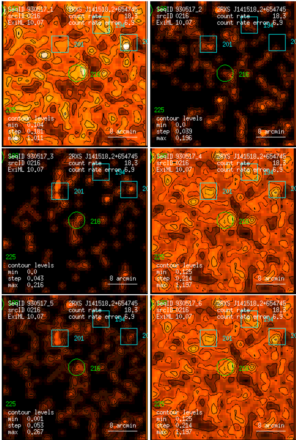
Figure 216: RASS 930517: detection 0216: band rate images, Gaussian filter: (1) PSPC channels 11 – 41, (2) 52 – 90, (3) 91 – 201, (4) 11 – 235, (5) 52 – 201, (6) 11 – 201. Broad band rates in counts/ks. Band rate contour levels in counts/ks/arcmin 2 .
