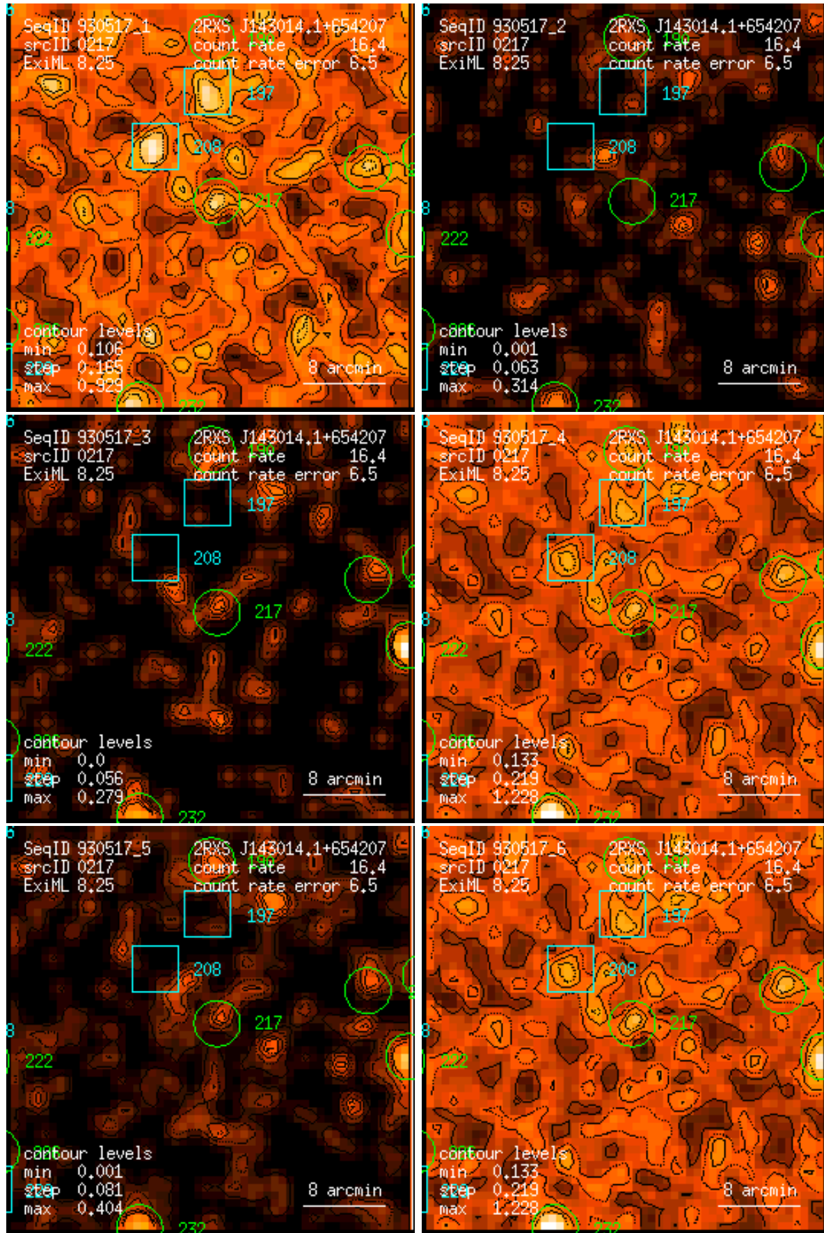
Figure 217: RASS 930517: detection 0217: band rate images, Gaussian filter: (1) PSPC channels 11 – 41, (2) 52 – 90, (3) 91 – 201, (4) 11 – 235, (5) 52 – 201, (6) 11 – 201. Broad band rates in counts/ks. Band rate contour levels in counts/ks/arcmin 2 .
