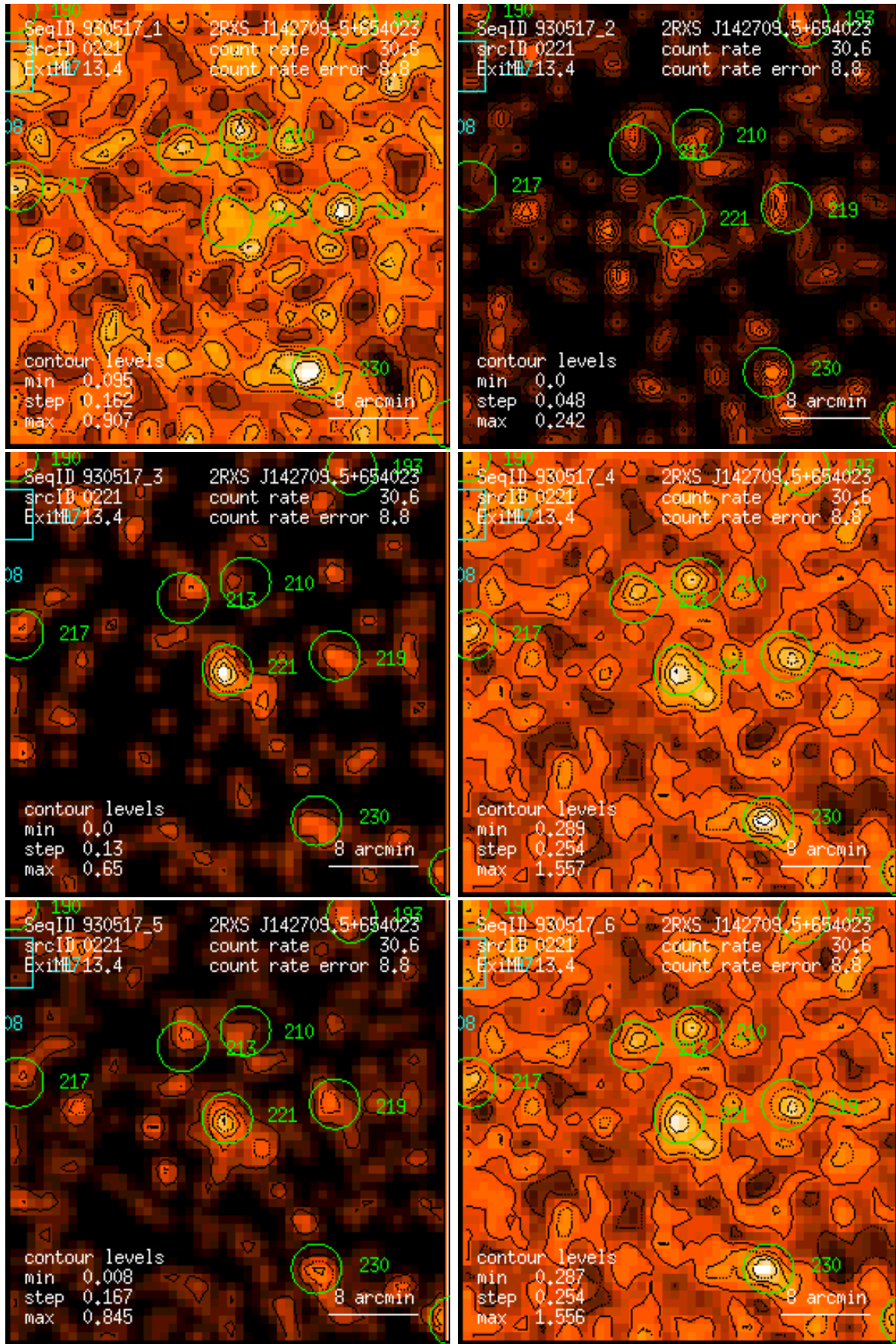
Figure 221: RASS 930517: detection 0221: band rate images, Gaussian filter: (1) PSPC channels 11 – 41, (2) 52 – 90, (3) 91 – 201, (4) 11 – 235, (5) 52 – 201, (6) 11 – 201. Broad band rates in counts/ks. Band rate contour levels in counts/ks/arcmin 2 .
