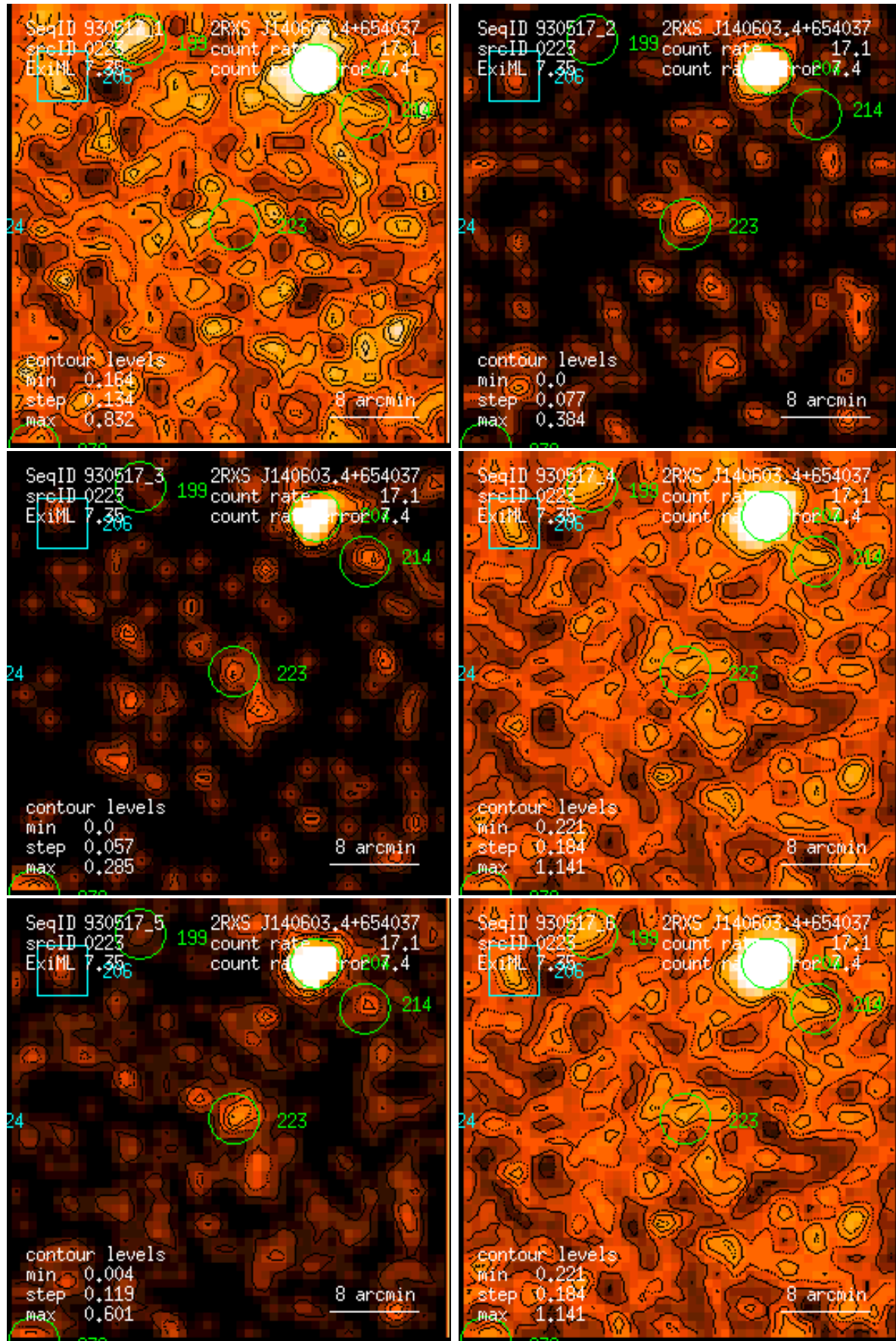
Figure 223: RASS 930517: detection 0223: band rate images, Gaussian filter: (1) PSPC channels 11 – 41, (2) 52 – 90, (3) 91 – 201, (4) 11 – 235, (5) 52 – 201, (6) 11 – 201. Broad band rates in counts/ks. Band rate contour levels in counts/ks/arcmin 2 .
