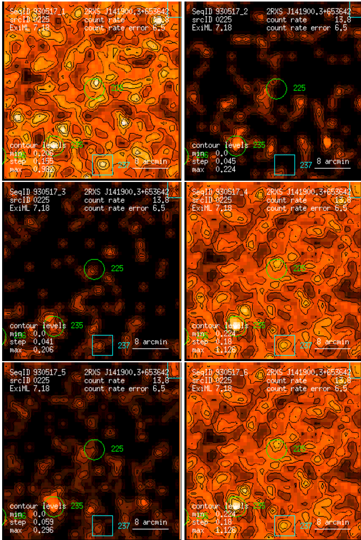
Figure 225: RASS 930517: detection 0225: band rate images, Gaussian filter: (1) PSPC channels 11 – 41, (2) 52 – 90, (3) 91 – 201, (4) 11 – 235, (5) 52 – 201, (6) 11 – 201. Broad band rates in counts/ks. Band rate contour levels in counts/ks/arcmin 2 .
