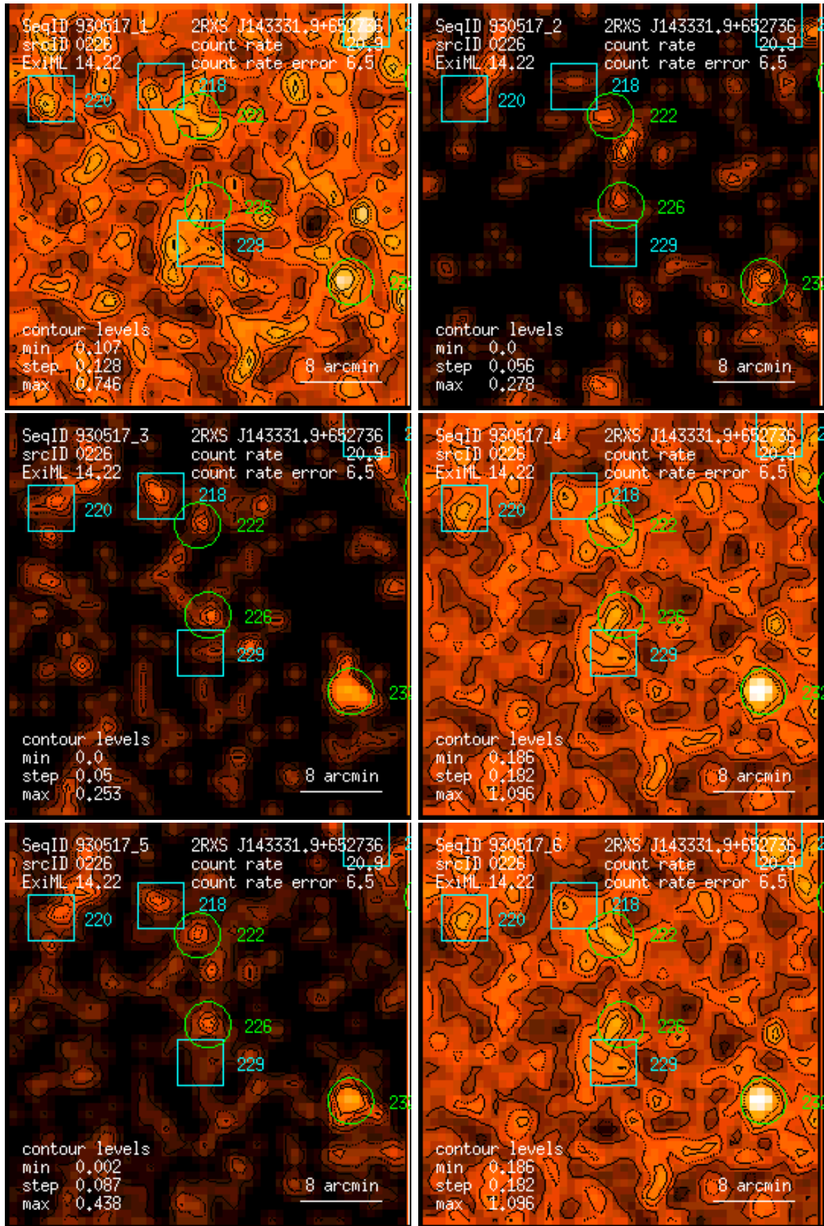
Figure 226: RASS 930517: detection 0226: band rate images, Gaussian filter: (1) PSPC channels 11 – 41, (2) 52 – 90, (3) 91 – 201, (4) 11 – 235, (5) 52 – 201, (6) 11 – 201. Broad band rates in counts/ks. Band rate contour levels in counts/ks/arcmin 2 .
