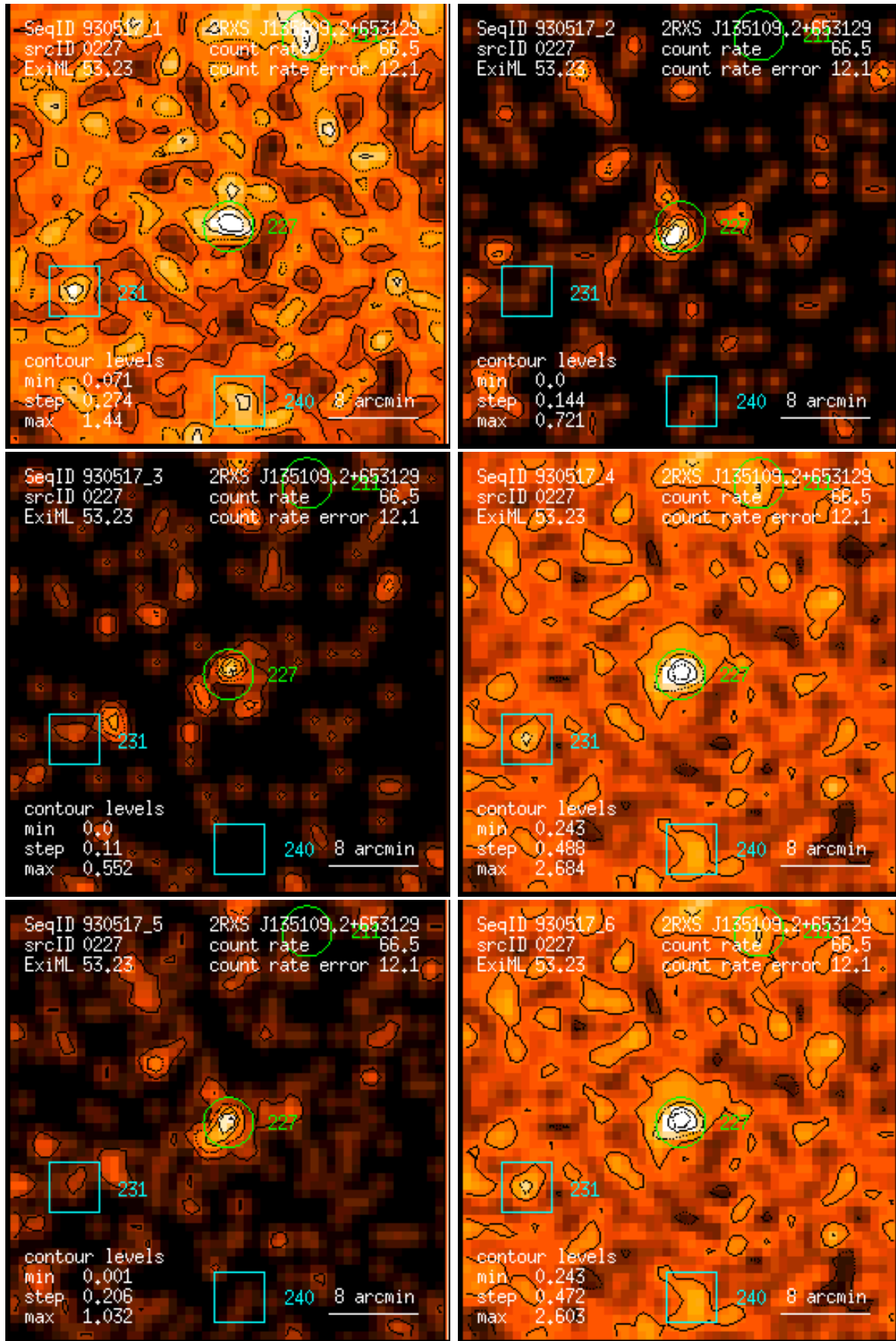
Figure 227: RASS 930517: detection 0227: band rate images, Gaussian filter: (1) PSPC channels 11 – 41, (2) 52 – 90, (3) 91 – 201, (4) 11 – 235, (5) 52 – 201, (6) 11 – 201. Broad band rates in counts/ks. Band rate contour levels in counts/ks/arcmin 2 .
