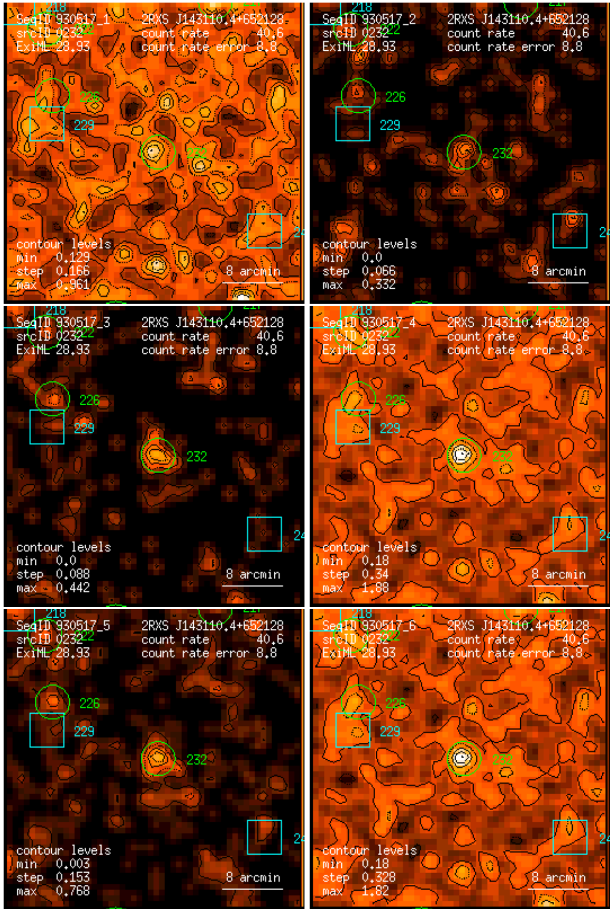
Figure 232: RASS 930517: detection 0232: band rate images, Gaussian filter: (1) PSPC channels 11 – 41, (2) 52 – 90, (3) 91 – 201, (4) 11 – 235, (5) 52 – 201, (6) 11 – 201. Broad band rates in counts/ks. Band rate contour levels in counts/ks/arcmin 2 .
