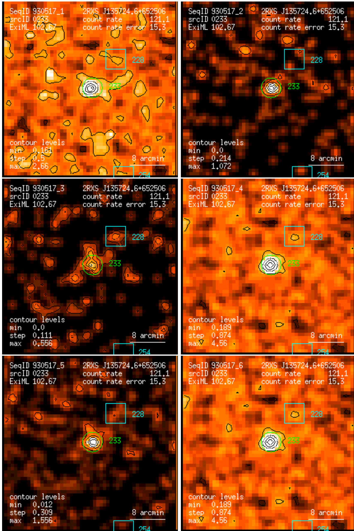
Figure 233: RASS 930517: detection 0233: band rate images, Gaussian filter: (1) PSPC channels 11 – 41, (2) 52 – 90, (3) 91 – 201, (4) 11 – 235, (5) 52 – 201, (6) 11 – 201. Broad band rates in counts/ks. Band rate contour levels in counts/ks/arcmin 2 .
