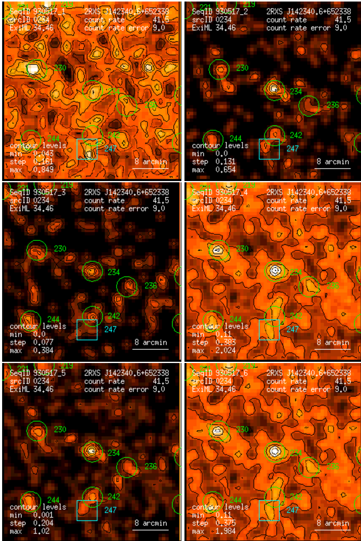
Figure 234: RASS 930517: detection 0234: band rate images, Gaussian filter: (1) PSPC channels 11 – 41, (2) 52 – 90, (3) 91 – 201, (4) 11 – 235, (5) 52 – 201, (6) 11 – 201. Broad band rates in counts/ks. Band rate contour levels in counts/ks/arcmin 2 .
