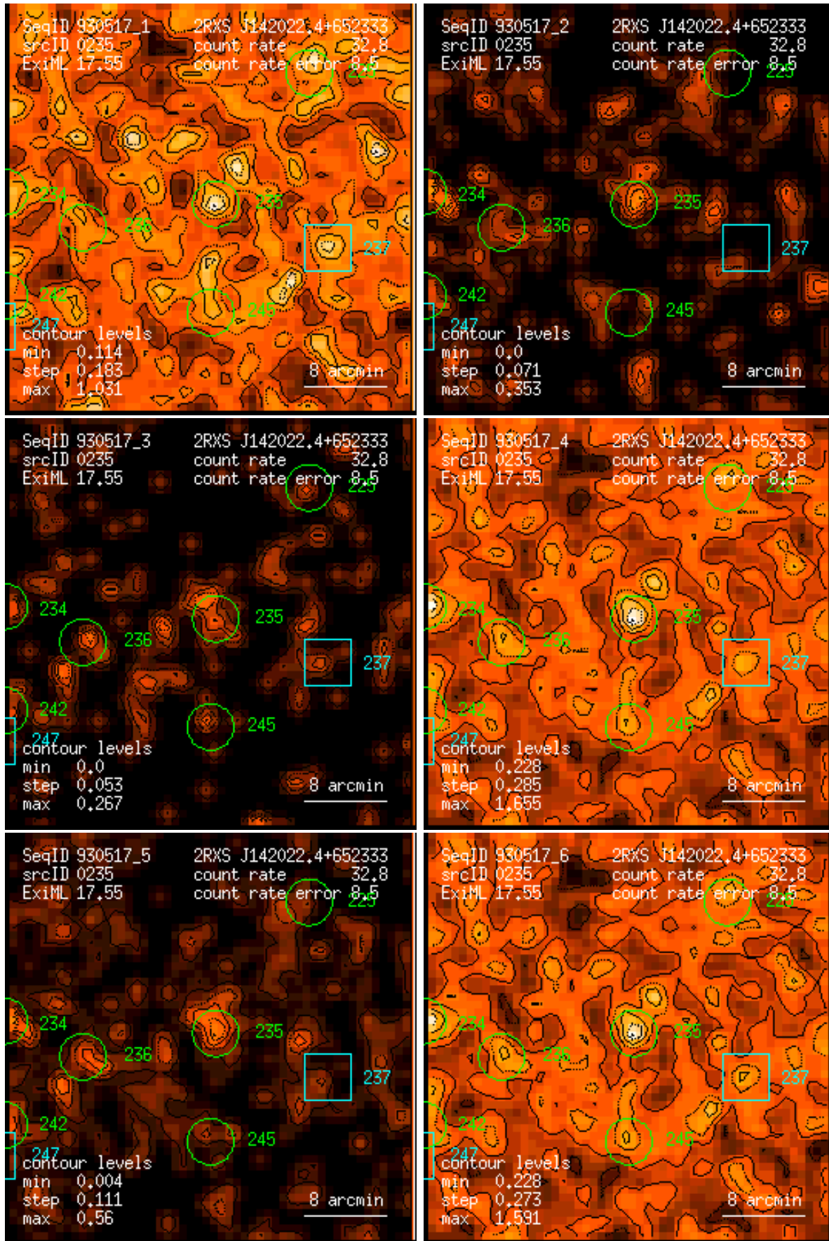
Figure 235: RASS 930517: detection 0235: band rate images, Gaussian filter: (1) PSPC channels 11 – 41, (2) 52 – 90, (3) 91 – 201, (4) 11 – 235, (5) 52 – 201, (6) 11 – 201. Broad band rates in counts/ks. Band rate contour levels in counts/ks/arcmin 2 .
