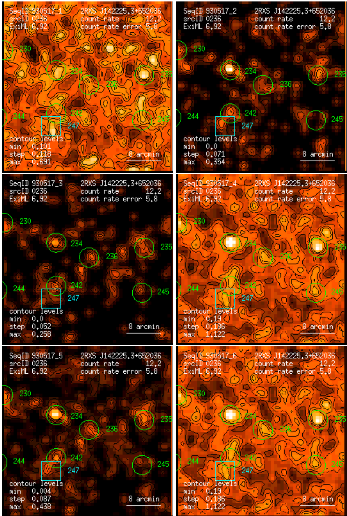
Figure 236: RASS 930517: detection 0236: band rate images, Gaussian filter: (1) PSPC channels 11 – 41, (2) 52 – 90, (3) 91 – 201, (4) 11 – 235, (5) 52 – 201, (6) 11 – 201. Broad band rates in counts/ks. Band rate contour levels in counts/ks/arcmin 2 .
