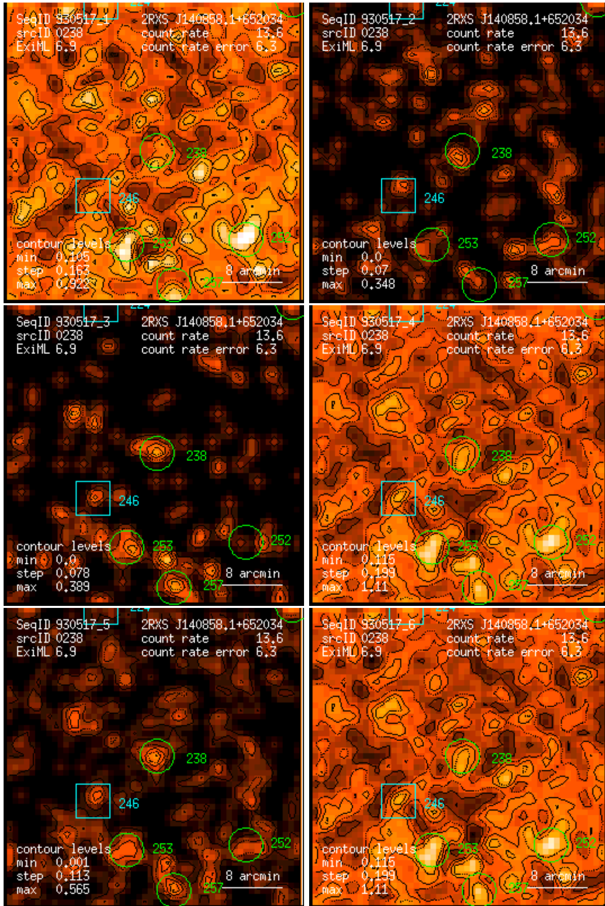
Figure 238: RASS 930517: detection 0238: band rate images, Gaussian filter: (1) PSPC channels 11 – 41, (2) 52 – 90, (3) 91 – 201, (4) 11 – 235, (5) 52 – 201, (6) 11 – 201. Broad band rates in counts/ks. Band rate contour levels in counts/ks/arcmin 2 .
