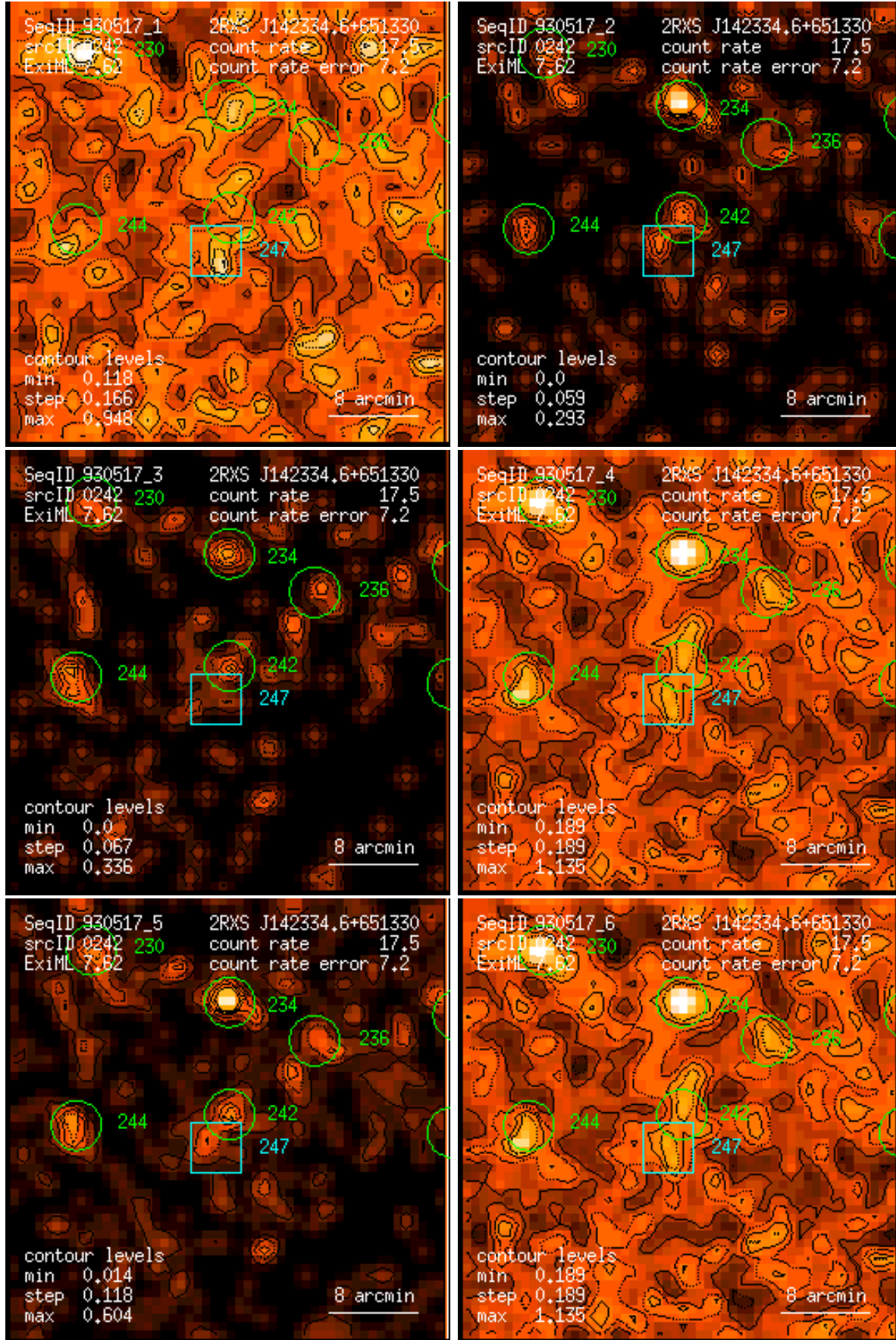
Figure 242: RASS 930517: detection 0242: band rate images, Gaussian filter: (1) PSPC channels 11 – 41, (2) 52 – 90, (3) 91 – 201, (4) 11 – 235, (5) 52 – 201, (6) 11 – 201. Broad band rates in counts/ks. Band rate contour levels in counts/ks/arcmin 2 .
