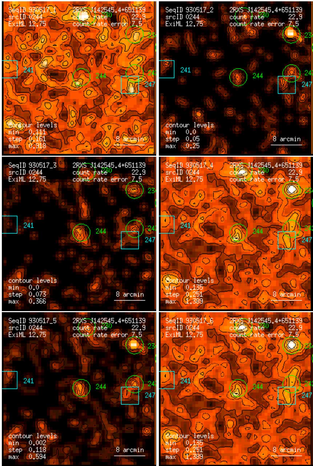
Figure 244: RASS 930517: detection 0244: band rate images, Gaussian filter: (1) PSPC channels 11 – 41, (2) 52 – 90, (3) 91 – 201, (4) 11 – 235, (5) 52 – 201, (6) 11 – 201. Broad band rates in counts/ks. Band rate contour levels in counts/ks/arcmin 2 .
