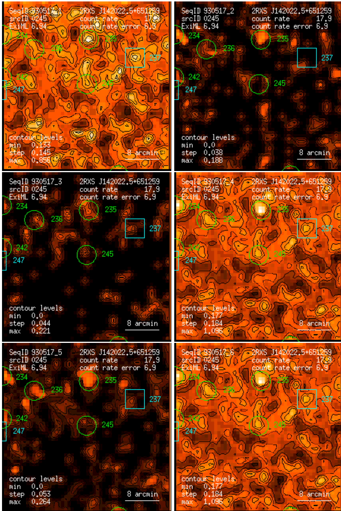
Figure 245: RASS 930517: detection 0245: band rate images, Gaussian filter: (1) PSPC channels 11 – 41, (2) 52 – 90, (3) 91 – 201, (4) 11 – 235, (5) 52 – 201, (6) 11 – 201. Broad band rates in counts/ks. Band rate contour levels in counts/ks/arcmin 2 .
