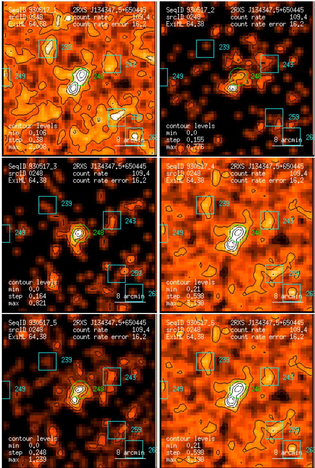
Figure 248: RASS 930517: detection 0248: band rate images, Gaussian filter: (1) PSPC channels 11 – 41, (2) 52 – 90, (3) 91 – 201, (4) 11 – 235, (5) 52 – 201, (6) 11 – 201. Broad band rates in counts/ks. Band rate contour levels in counts/ks/arcmin 2 .
