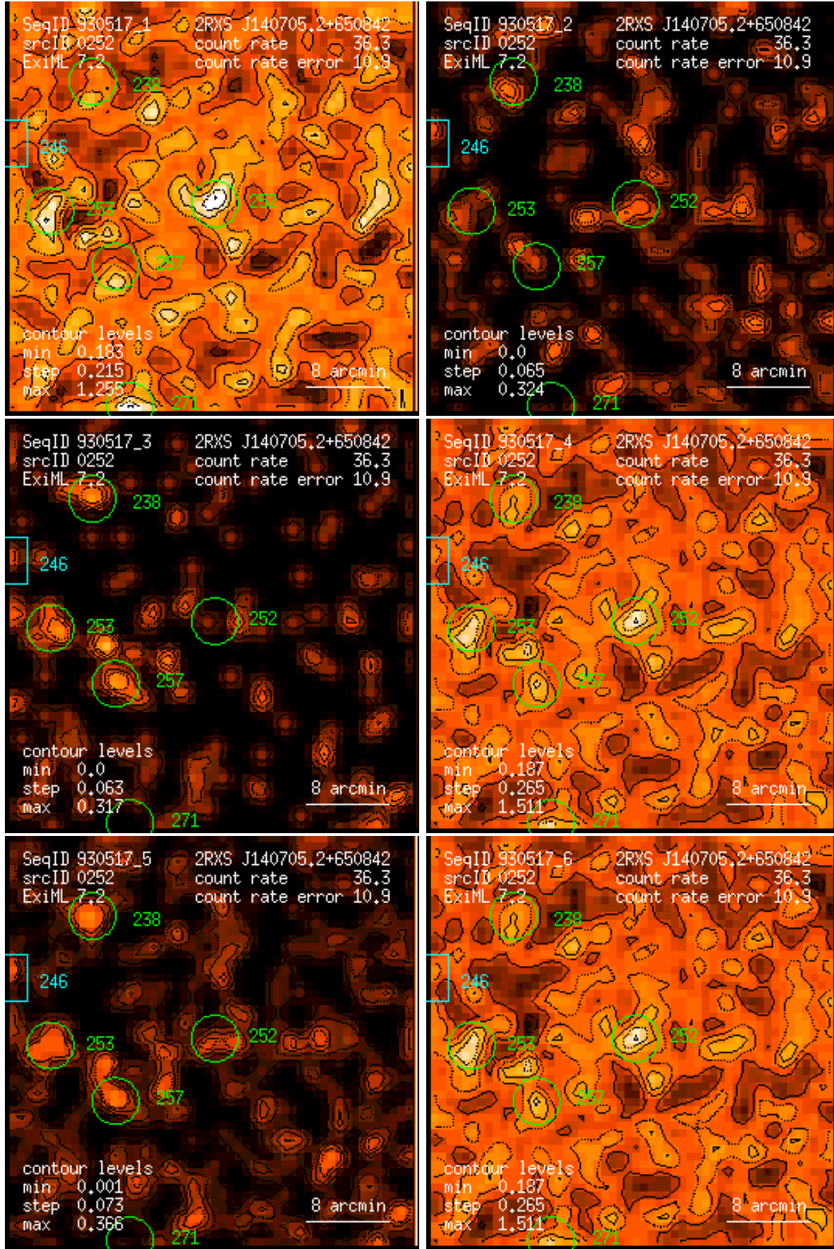
Figure 252: RASS 930517: detection 0252: band rate images, Gaussian filter: (1) PSPC channels 11 – 41, (2) 52 – 90, (3) 91 – 201, (4) 11 – 235, (5) 52 – 201, (6) 11 – 201. Broad band rates in counts/ks. Band rate contour levels in counts/ks/arcmin 2 .
