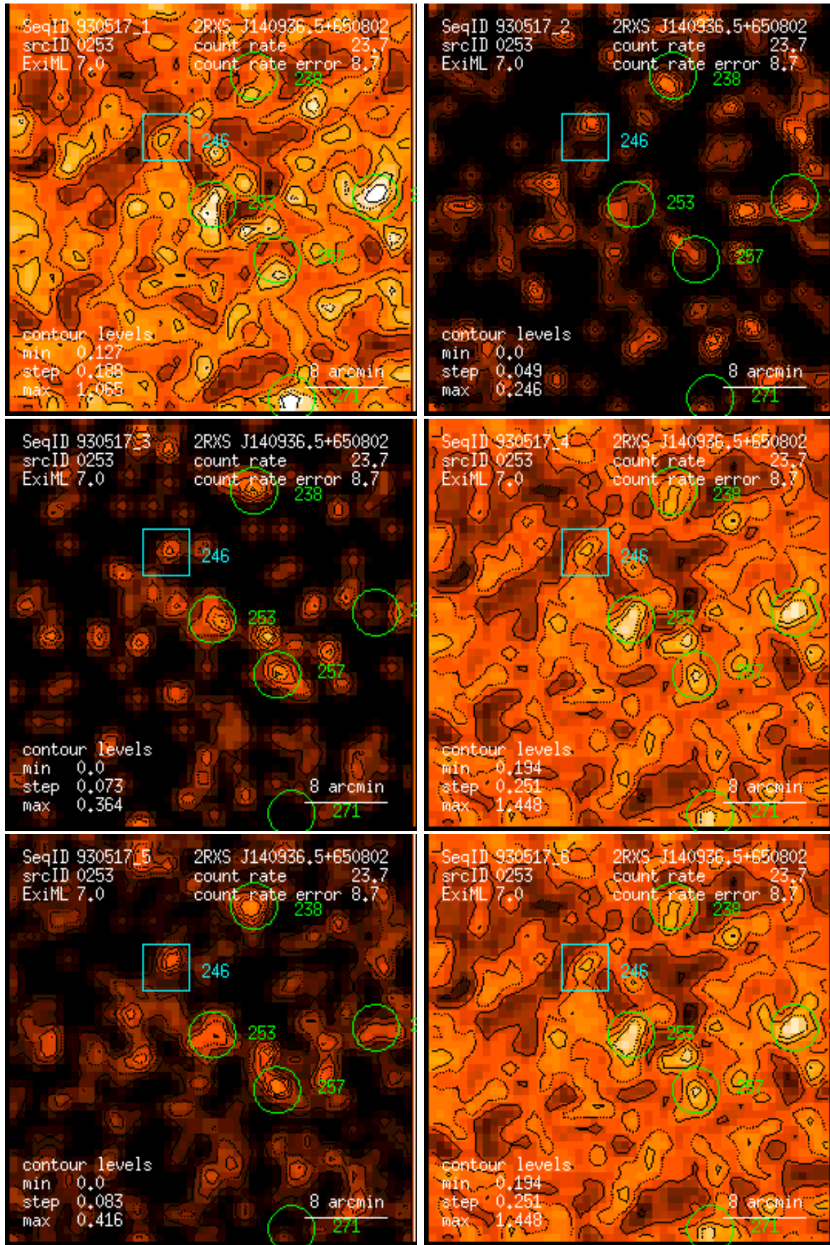
Figure 253: RASS 930517: detection 0253: band rate images, Gaussian filter: (1) PSPC channels 11 – 41, (2) 52 – 90, (3) 91 – 201, (4) 11 – 235, (5) 52 – 201, (6) 11 – 201. Broad band rates in counts/ks. Band rate contour levels in counts/ks/arcmin 2 .
