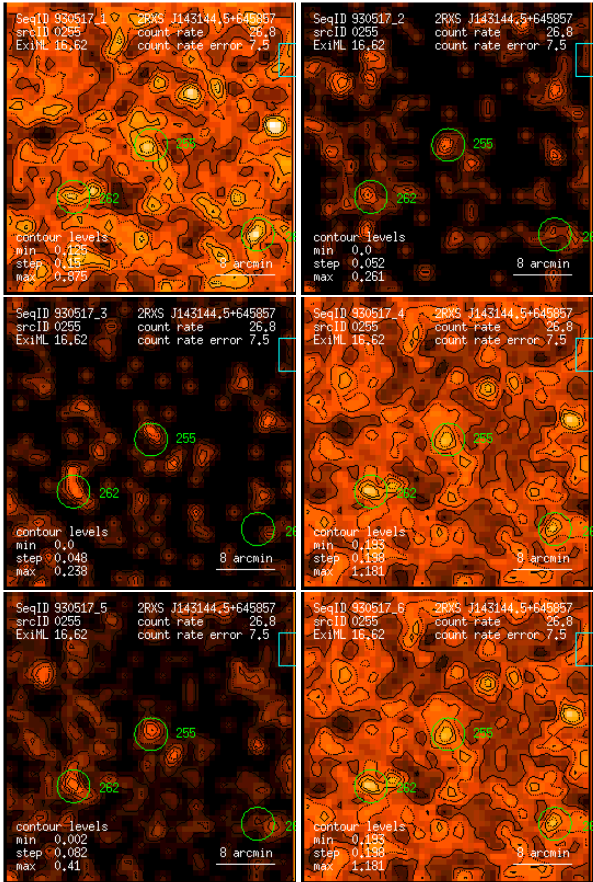
Figure 255: RASS 930517: detection 0255: band rate images, Gaussian filter: (1) PSPC channels 11 – 41, (2) 52 – 90, (3) 91 – 201, (4) 11 – 235, (5) 52 – 201, (6) 11 – 201. Broad band rates in counts/ks. Band rate contour levels in counts/ks/arcmin 2 .
