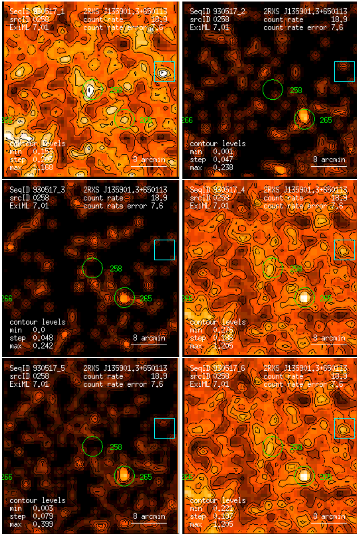
Figure 258: RASS 930517: detection 0258: band rate images, Gaussian filter: (1) PSPC channels 11 – 41, (2) 52 – 90, (3) 91 – 201, (4) 11 – 235, (5) 52 – 201, (6) 11 – 201. Broad band rates in counts/ks. Band rate contour levels in counts/ks/arcmin 2 .
