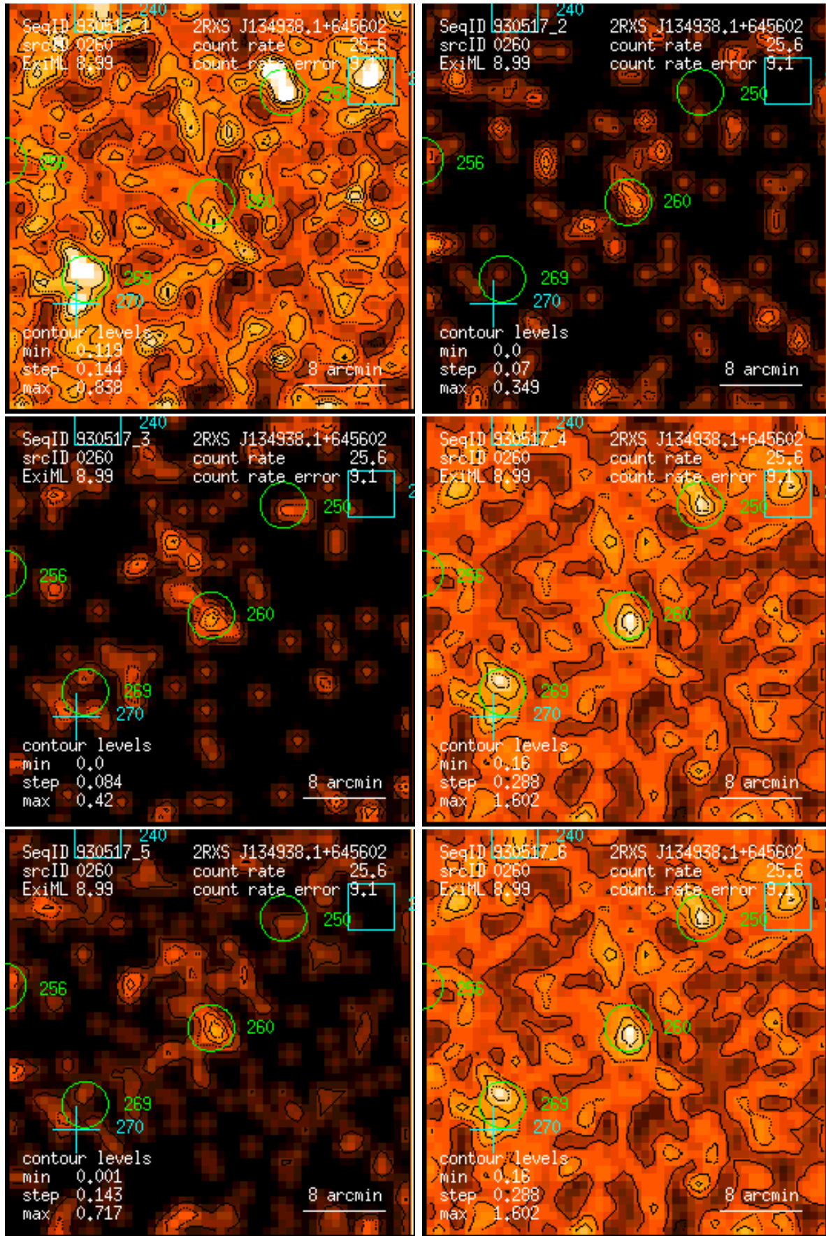
Figure 260: RASS 930517: detection 0260: band rate images, Gaussian filter: (1) PSPC channels 11 – 41, (2) 52 – 90, (3) 91 – 201, (4) 11 – 235, (5) 52 – 201, (6) 11 – 201. Broad band rates in counts/ks. Band rate contour levels in counts/ks/arcmin 2 .
