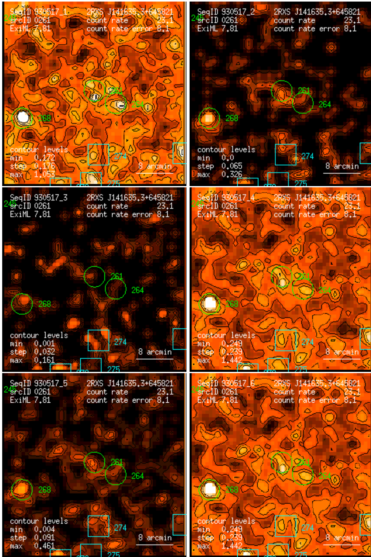
Figure 261: RASS 930517: detection 0261: band rate images, Gaussian filter: (1) PSPC channels 11 – 41, (2) 52 – 90, (3) 91 – 201, (4) 11 – 235, (5) 52 – 201, (6) 11 – 201. Broad band rates in counts/ks. Band rate contour levels in counts/ks/arcmin 2 .
