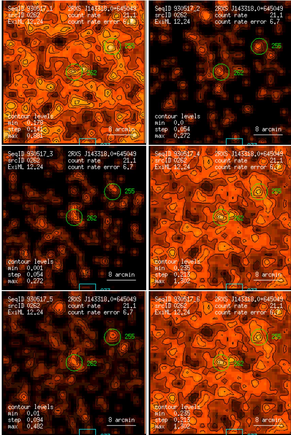
Figure 262: RASS 930517: detection 0262: band rate images, Gaussian filter: (1) PSPC channels 11 – 41, (2) 52 – 90, (3) 91 – 201, (4) 11 – 235, (5) 52 – 201, (6) 11 – 201. Broad band rates in counts/ks. Band rate contour levels in counts/ks/arcmin 2 .
