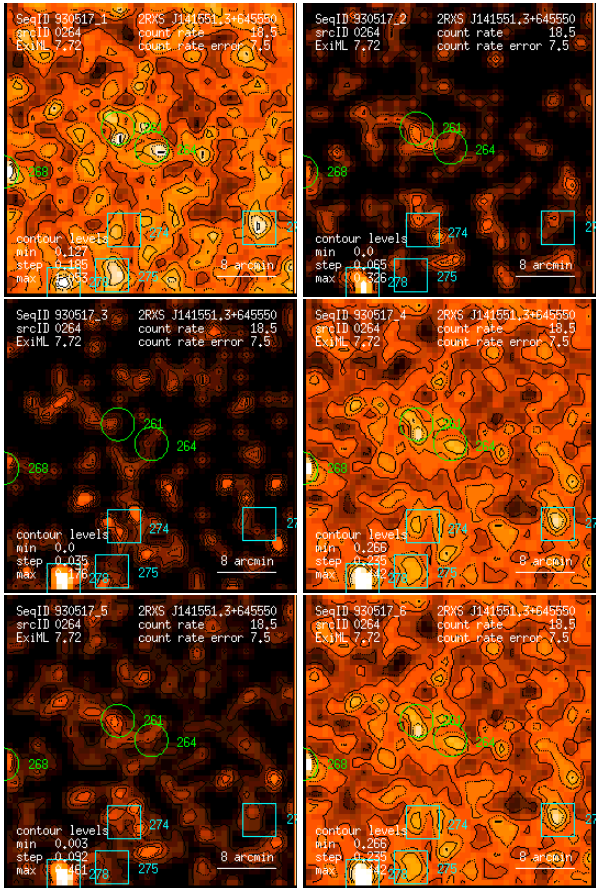
Figure 264: RASS 930517: detection 0264: band rate images, Gaussian filter: (1) PSPC channels 11 – 41, (2) 52 – 90, (3) 91 – 201, (4) 11 – 235, (5) 52 – 201, (6) 11 – 201. Broad band rates in counts/ks. Band rate contour levels in counts/ks/arcmin 2 .
