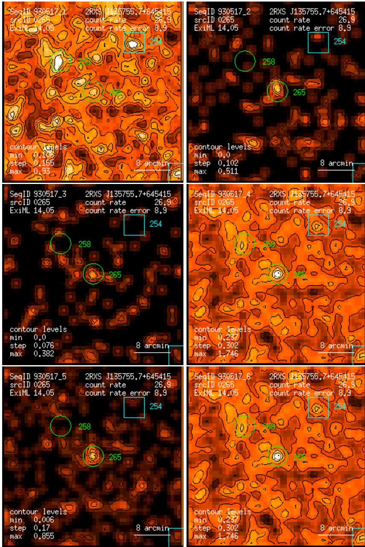
Figure 265: RASS 930517: detection 0265: band rate images, Gaussian filter: (1) PSPC channels 11 – 41, (2) 52 – 90, (3) 91 – 201, (4) 11 – 235, (5) 52 – 201, (6) 11 – 201. Broad band rates in counts/ks. Band rate contour levels in counts/ks/arcmin 2 .
