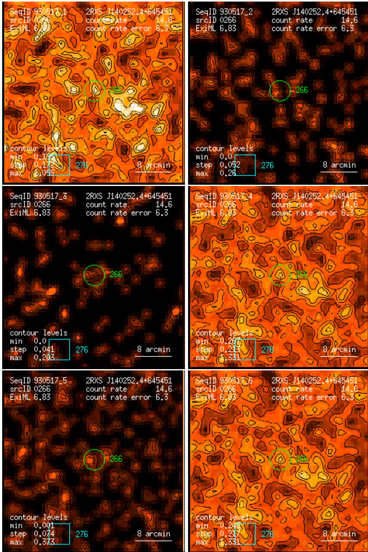
Figure 266: RASS 930517: detection 0266: band rate images, Gaussian filter: (1) PSPC channels 11 – 41, (2) 52 – 90, (3) 91 – 201, (4) 11 – 235, (5) 52 – 201, (6) 11 – 201. Broad band rates in counts/ks. Band rate contour levels in counts/ks/arcmin 2 .
