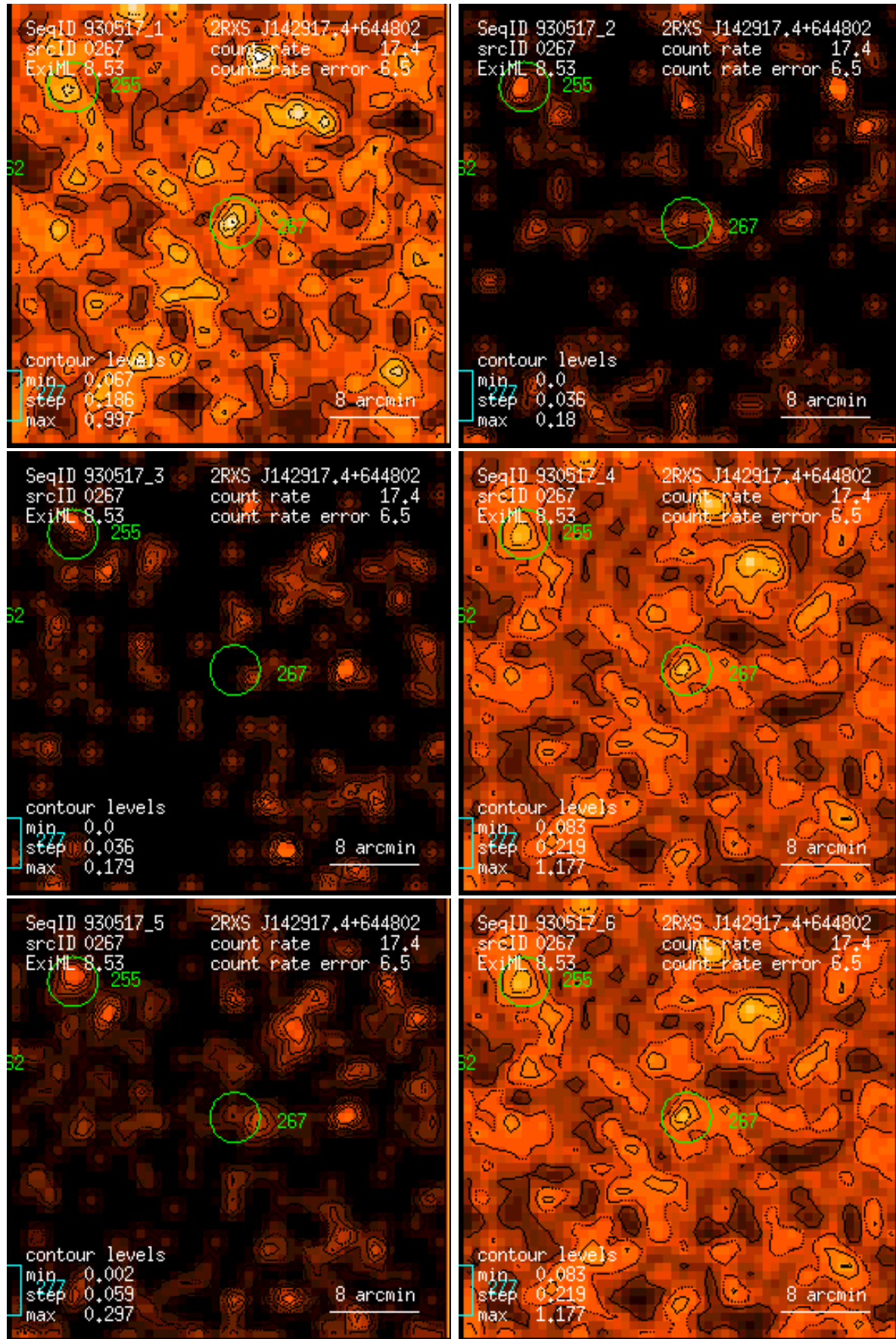
Figure 267: RASS 930517: detection 0267: band rate images, Gaussian filter: (1) PSPC channels 11 – 41, (2) 52 – 90, (3) 91 – 201, (4) 11 – 235, (5) 52 – 201, (6) 11 – 201. Broad band rates in counts/ks. Band rate contour levels in counts/ks/arcmin 2 .
