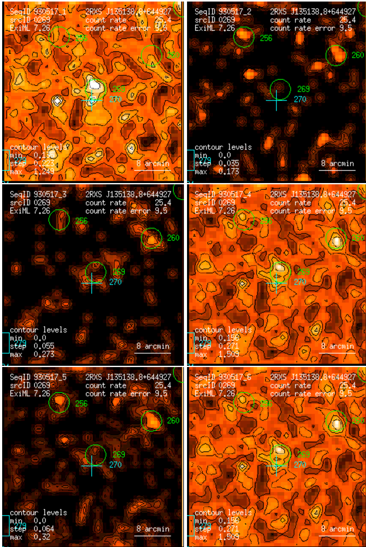
Figure 269: RASS 930517: detection 0269: band rate images, Gaussian filter: (1) PSPC channels 11 – 41, (2) 52 – 90, (3) 91 – 201, (4) 11 – 235, (5) 52 – 201, (6) 11 – 201. Broad band rates in counts/ks. Band rate contour levels in counts/ks/arcmin 2 .
