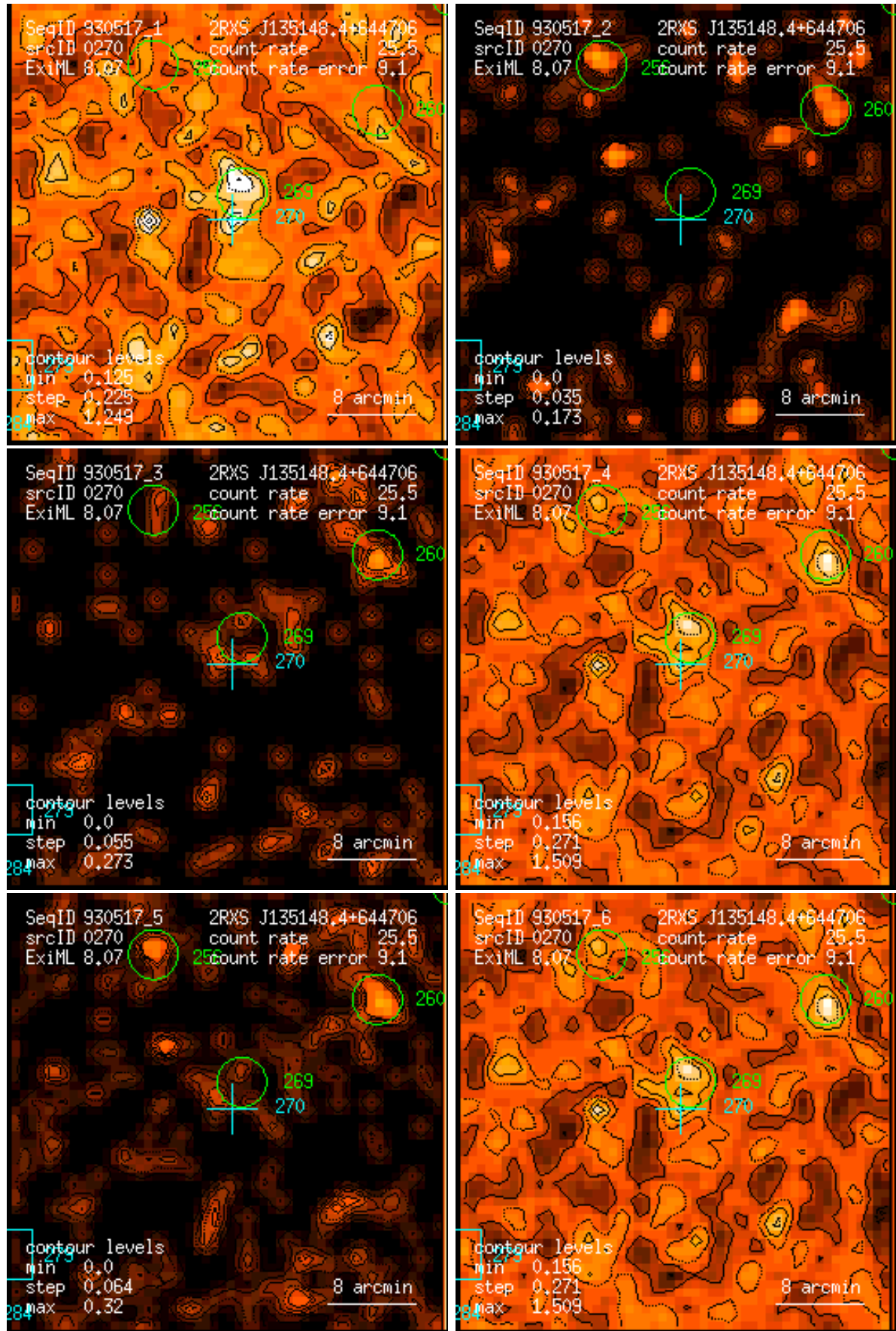
Figure 270: RASS 930517: detection 0270: band rate images, Gaussian filter: (1) PSPC channels 11 – 41, (2) 52 – 90, (3) 91 – 201, (4) 11 – 235, (5) 52 – 201, (6) 11 – 201. Broad band rates in counts/ks. Band rate contour levels in counts/ks/arcmin 2 .
