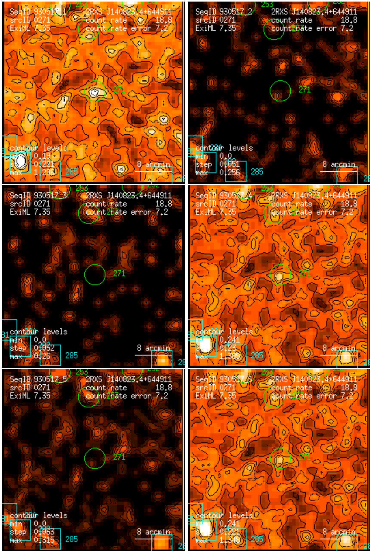
Figure 271: RASS 930517: detection 0271: band rate images, Gaussian filter: (1) PSPC channels 11 – 41, (2) 52 – 90, (3) 91 – 201, (4) 11 – 235, (5) 52 – 201, (6) 11 – 201. Broad band rates in counts/ks. Band rate contour levels in counts/ks/arcmin 2 .
