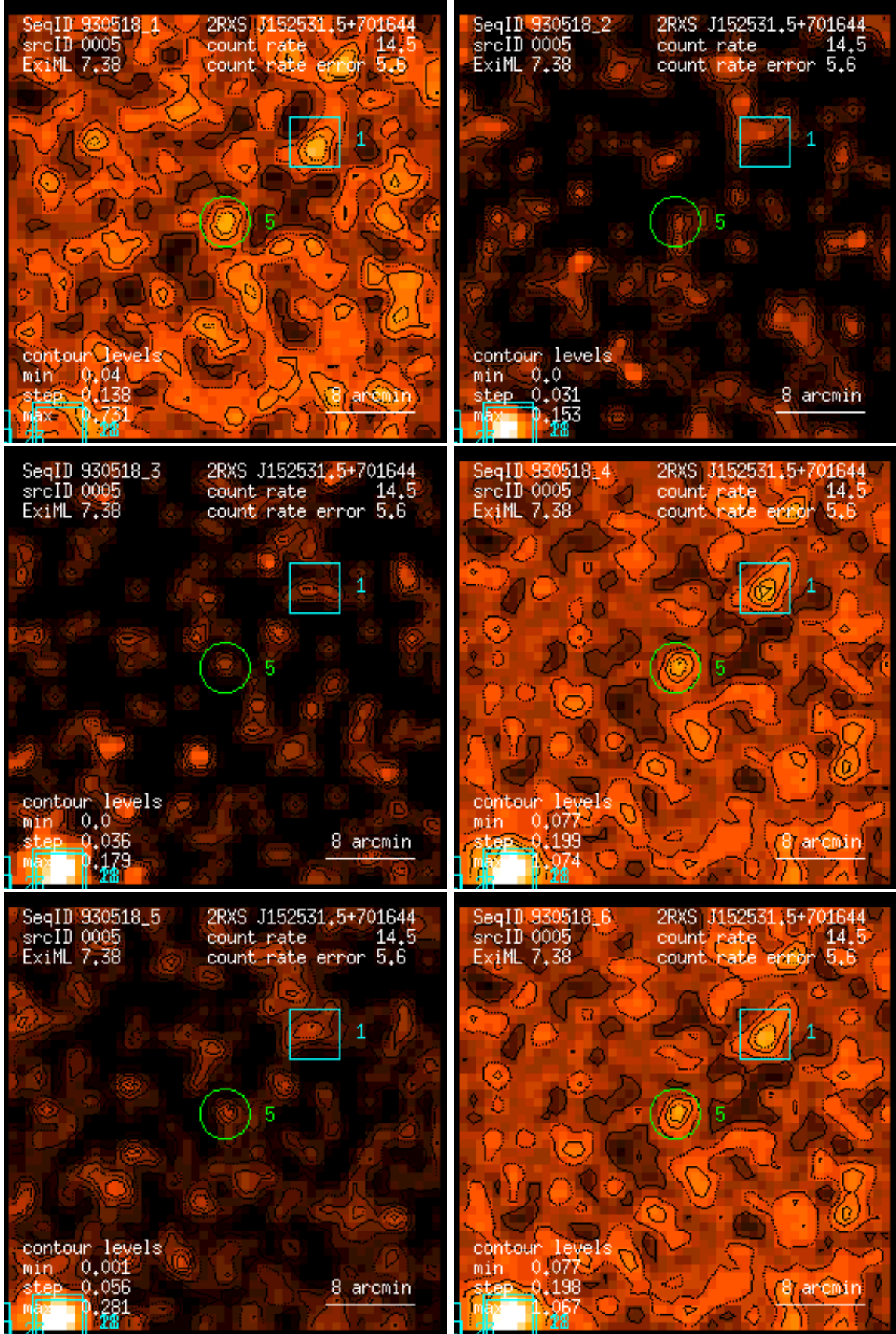
Figure 5: RASS 930518: detection 0005: band rate images, Gaussian filter: (1) PSPC channels 11 – 41, (2) 52 – 90, (3) 91 – 201, (4) 11 – 235, (5) 52 – 201, (6) 11 – 201. Broad band rates in counts/ks. Band rate contour levels in counts/ks/arcmin 2 .
