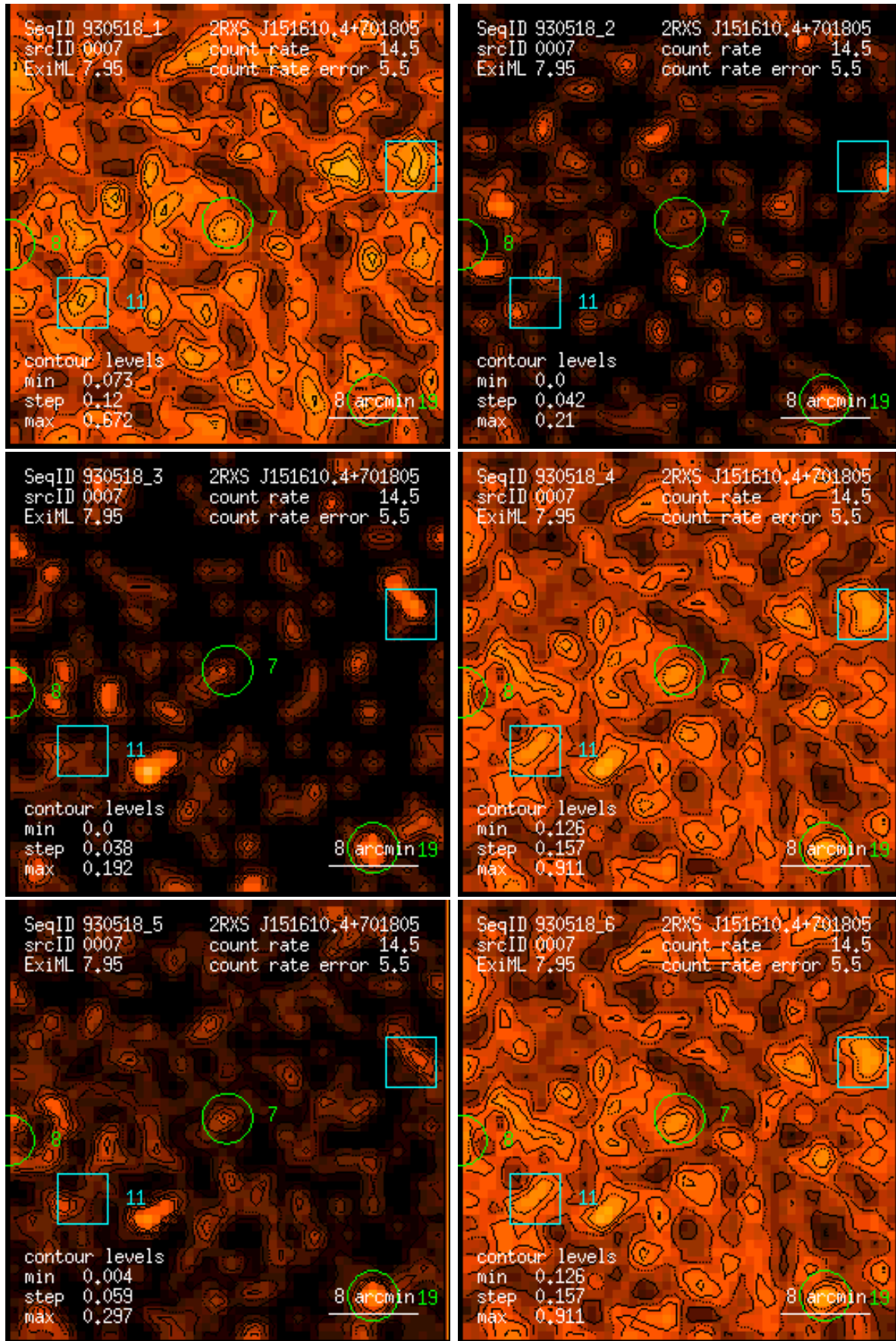
Figure 7: RASS 930518: detection 0007: band rate images, Gaussian filter: (1) PSPC channels 11 – 41, (2) 52 – 90, (3) 91 – 201, (4) 11 – 235, (5) 52 – 201, (6) 11 – 201. Broad band rates in counts/ks. Band rate contour levels in counts/ks/arcmin 2 .
