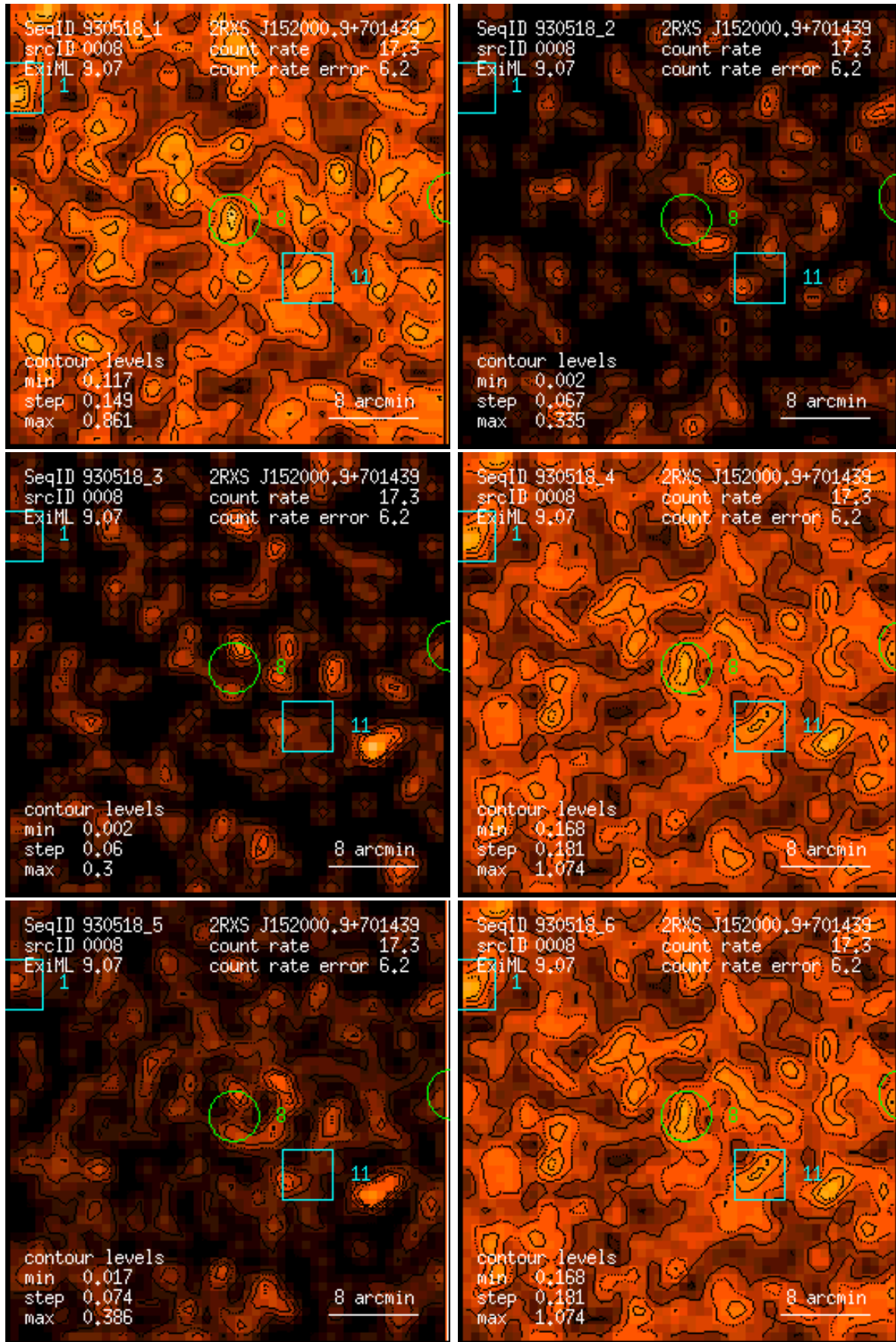
Figure 8: RASS 930518: detection 0008: band rate images, Gaussian filter: (1) PSPC channels 11 – 41, (2) 52 – 90, (3) 91 – 201, (4) 11 – 235, (5) 52 – 201, (6) 11 – 201. Broad band rates in counts/ks. Band rate contour levels in counts/ks/arcmin 2 .
